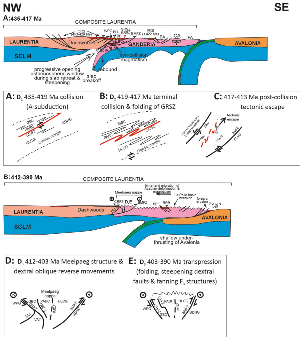
Fig. 10. Tectonic models for Salinic (A) and Acadian (B) orogenies modified from van Staal and Barr (2012) and van Staal et al. (2014a). The sketches presented in A–E represent cross-sectional cartoons depicting the progression in tectonic settings from D1 to D3 of the collision between the Gander margin and composite Laurentia. (A) D1 (Salinic) underthrusting of the Gander margin (A-subduction) with shear localized in the GRSZ and folding and foliation development in the adjacent rocks; (B) D1 progressed into D2 structural thickening in the Salinic collision zone, which leads to folding of the GRSZ. Granite intrusion and peak temperature Barrovian metamorphism characterize the terminal stage of D2; (C) Post 417 Ma tectonic escape of a wedge of high-grade rocks towards the southeast such that the HLCG is thrust over the BDNG. The tectonites preserved between the CRFZ and GBFZ accommodated pre-D3 normal sense of motion with respect to their hangingwall, which is now inferred to be buried beneath the leading western edge of the Meelapaeg structure; (D) Early stage of D3 (Acadian) bi-vergent Meelapaeg structure development with reverse shear strain localized in shear zones such as the CRFZ and BMFZ. Northwestward-dipping D2 tectonites involved in the preceding tectonic escape between the CRFZ and GBFZ progressively rotate and acquire a southeasterly dip; (E) F3 folding and progressive D3 steepening of the shear zones formed during Meelapaeg structure formation. The steepened shear zones acquire a favourable orientation to accommodate dextral strike-slip motions. The timing of the various stages is approximate and/or interpretative, and in part based on existing constraints concerning the start and end of the Salinic collision in southern Newfoundland (see text). Most abbreviations are given in text and previous figures. BB, Badger–Botwood basin; BA, backarc to coastal arc (CA); BEF, Bay d’Est Fault; FA, forearc to coastal arc; ORS, Old Red Sandstone and related terrestrial rocks in red, which become progressively younger southeastwards; RRB, Rocky Ridge basin; VA, Victoria arc; WPG, Windsor Point Group.
