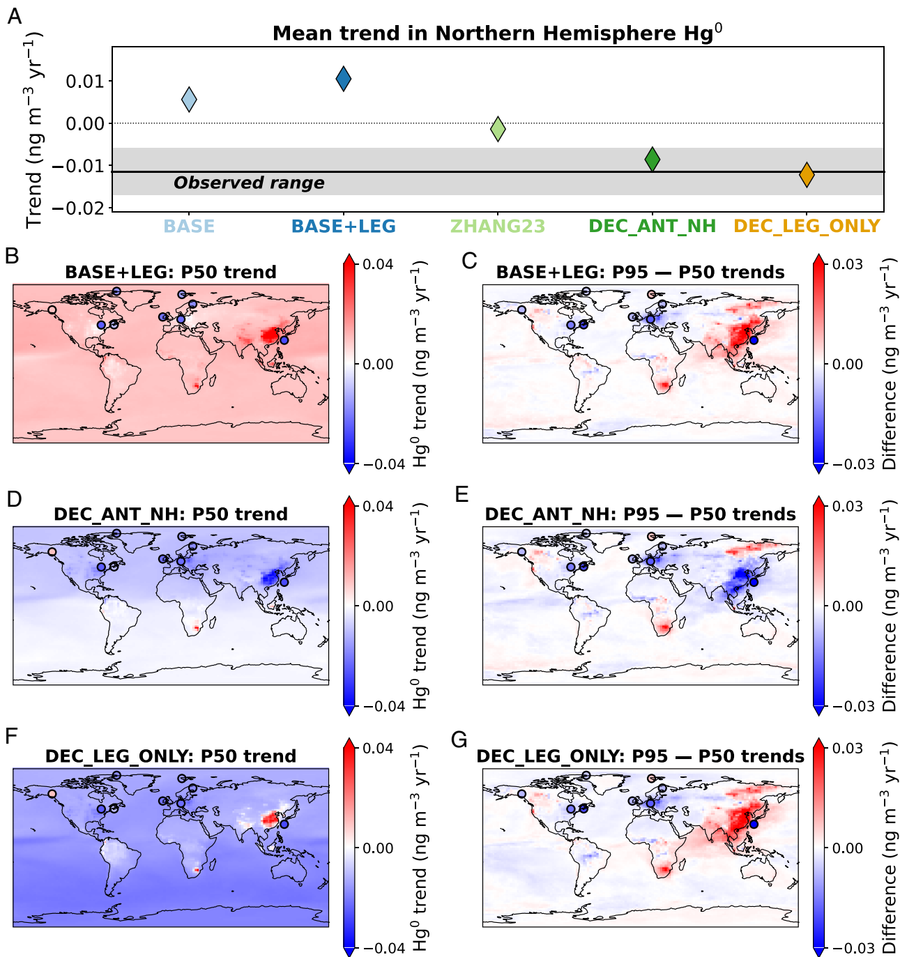
Fig. 4. Comparison between trends (2005 to 2020) in GEOS-Chem model simulations and observations for NH mean Hg^0 (A), calculated using linear mixed effects modeling of available NH regions and calculating the area-weighted mean (Fig. 2). The observed range in the NH Hg^0 trend is shown as a black line (mean) with shaded area ( \pm 2\sigma ). Error bars are smaller than the markers for the model simulations. Maps show BASE+LEG trends in median (P50) daily deseasonalized simulated values (B), BASE+LEG differences between the 95th percentile (P95) trend and median (P50) trend (C), DEC_ANT_NH P50 trends (D), DEC_ANT_NH differences between P95 and P50 trends (E), DEC_LEG_ONLY P50 trends (F), DEC_LEG_ONLY differences between P95 and P50 trends (G). BASE+LEG is the simulation with Streets et al. (10) emissions and associated legacy feedbacks, DEC_ANT_NH is the simulation with decreasing anthropogenic emissions in the NH, and DEC_LEG_ONLY includes a decline in legacy emissions from the ocean (Table 1). Observed results are plotted in filled circles for 9 stations with more than 13 y of high-frequency data. The other simulations are shown in SI Appendix, Fig. S13 .
