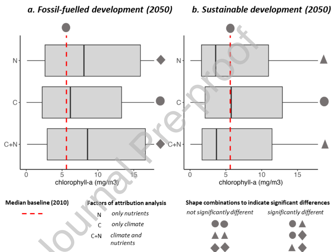
Figure 3: Attribution analysis of nutrient and climate factors on the median chlorophyll-a concentration ( \text{mg}/\text{m}^3 ) in (a) the fossil-fuelled development scenario and (b) the sustainable development scenario for the year 2050. The attribution is relative to the baseline for the year 2010 (red dashed line). N refers to nutrient factors. C refers to climate factors. N+C refers to the interaction effect of nutrient and climate factors. The shapes on the right side of each bar indicate whether the factors had a significant impact (e.g., circle and diamond) or not (e.g., two triangles) compared to the other scenarios. We used a pairwise permutation test to test significance, P < 0.05 (see Section 2.5 for details on the attribution analysis).
