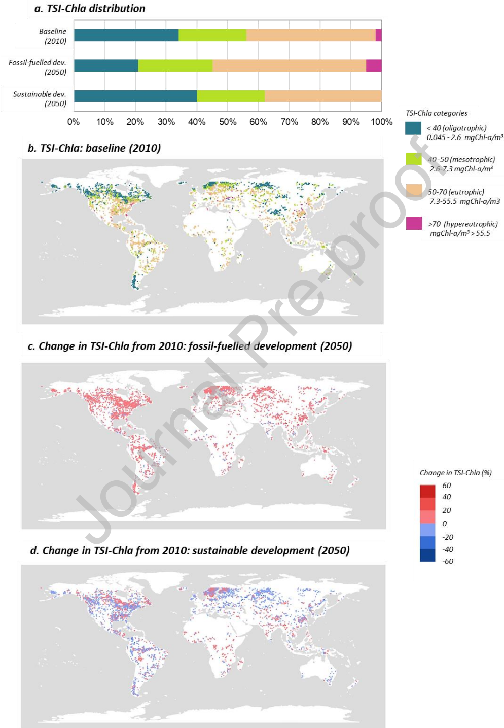
Figure 2: Projected changes in Trophic State Index for chlorophyll-a (TSI-Chla) for representative lakes in 2050 scenarios compared to the baseline of 2010. a. distribution of TSI-Chla in the scenarios. b. TSI-Chla calculations for the baseline (2010). c. projected change in TSI-Chla in the fossil-fuelled development scenario for 2050. d. projected change in TSI-Chla in the sustainable development scenario for 2050. Chl-a is short for chlorophyll-a.
