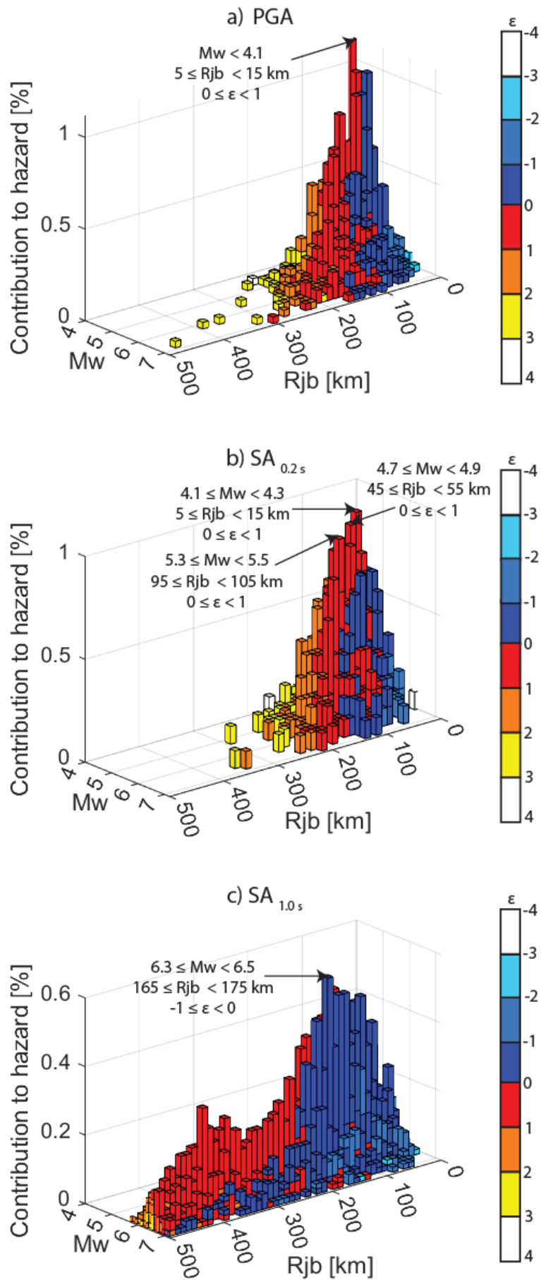
Figure 45: Disaggregation of the hazard for the Acorn site and 2475-year return period by magnitude ( M_w ), Joyner-Boore distance ( R_{jb} ) and epsilon ( \epsilon ) for (a) PGA, (b) SA 0.2s , and (c) SA 1.0s .
