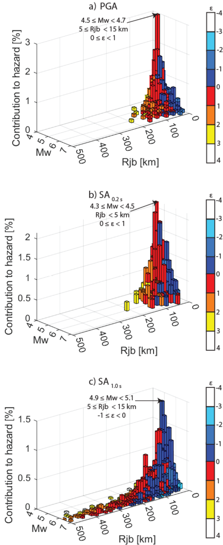
Figure 47: Disaggregation of the hazard for the Endurance site and 2475-year return period by magnitude ( M_w ), Joyner-Boore distance ( R_{jb} ) and epsilon ( \epsilon ) for (a) PGA, (b) SA_{0.2s} , and (c) SA_{1.0s} .
