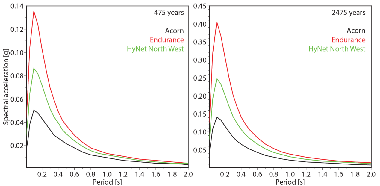
Figure 43: UHS for return periods of 475 years and 2475 years for the sites shown in Figure 42.
