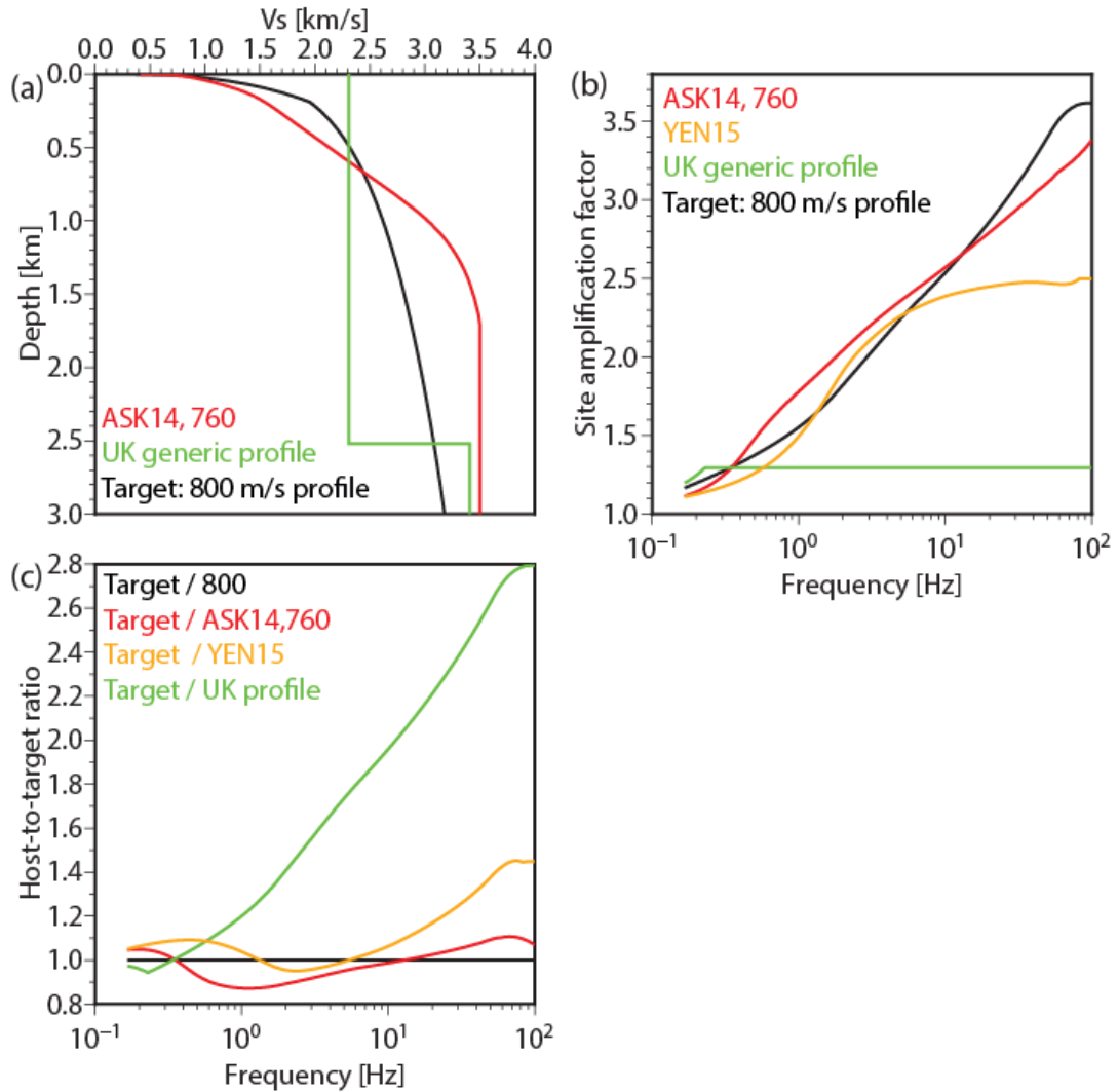
Figure 35: (a) Target and host Vs profiles used for the five GMPEs in Table 8. (b) Target and host site amplification factors used for the FAS of each GMPE. (c) Host-to-target amplification ratios.
