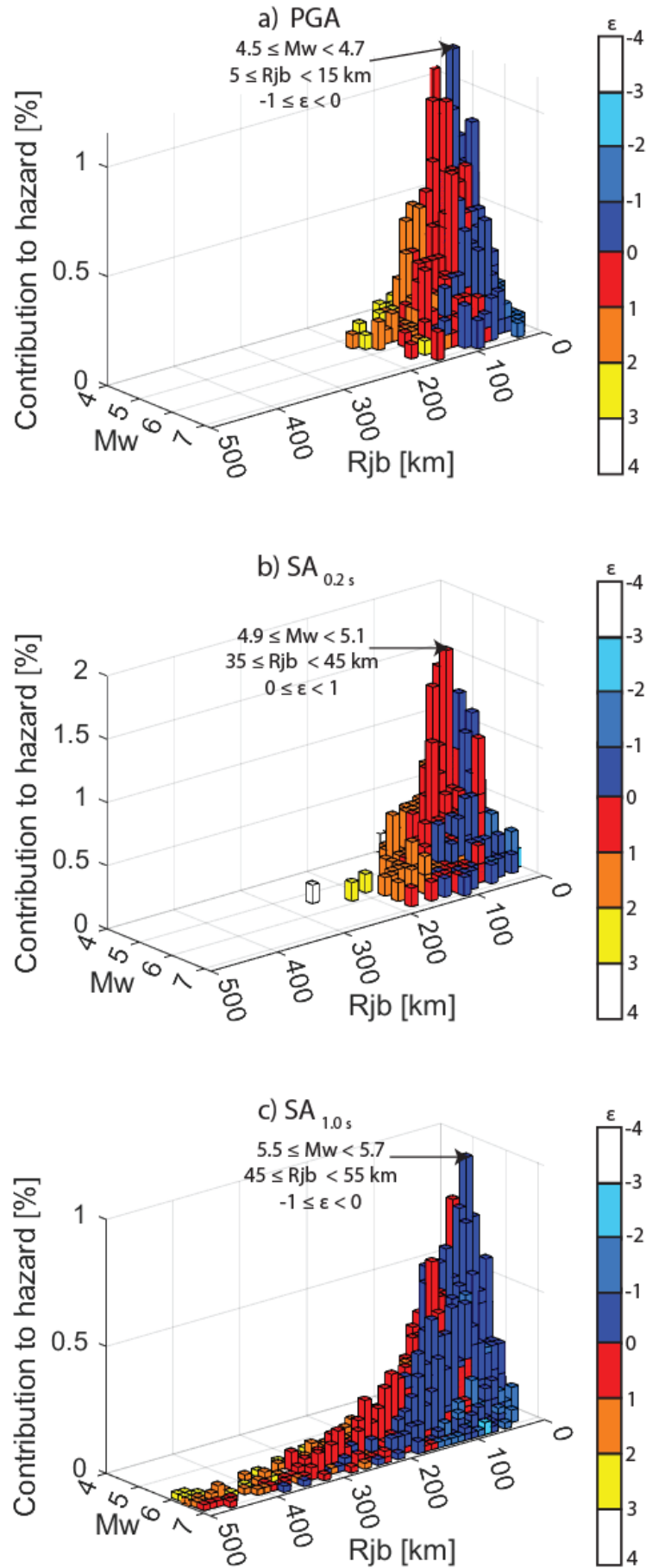
Figure 49: Disaggregation of the hazard for the HyNet site and 2475-year return period by magnitude ( M_w ), Joyner-Boore distance ( R_{jb} ) and epsilon ( \epsilon ) for (a) PGA, (b) SA_{0.2s} , and (c) SA_{1.0s} .
