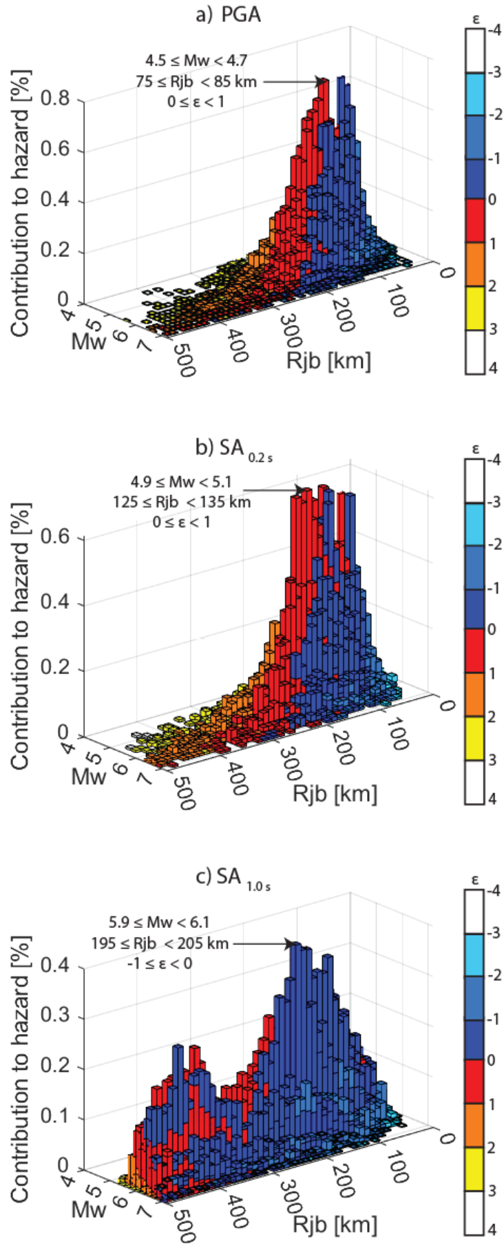
Figure 44: Disaggregation of the hazard for the Acorn site and 475-year return period by magnitude ( M_w ), Joyner-Boore distance ( R_{jb} ) and epsilon ( \epsilon ) for (a) PGA, (b) SA_{0.2s} , and (c) SA_{1.0s} .
