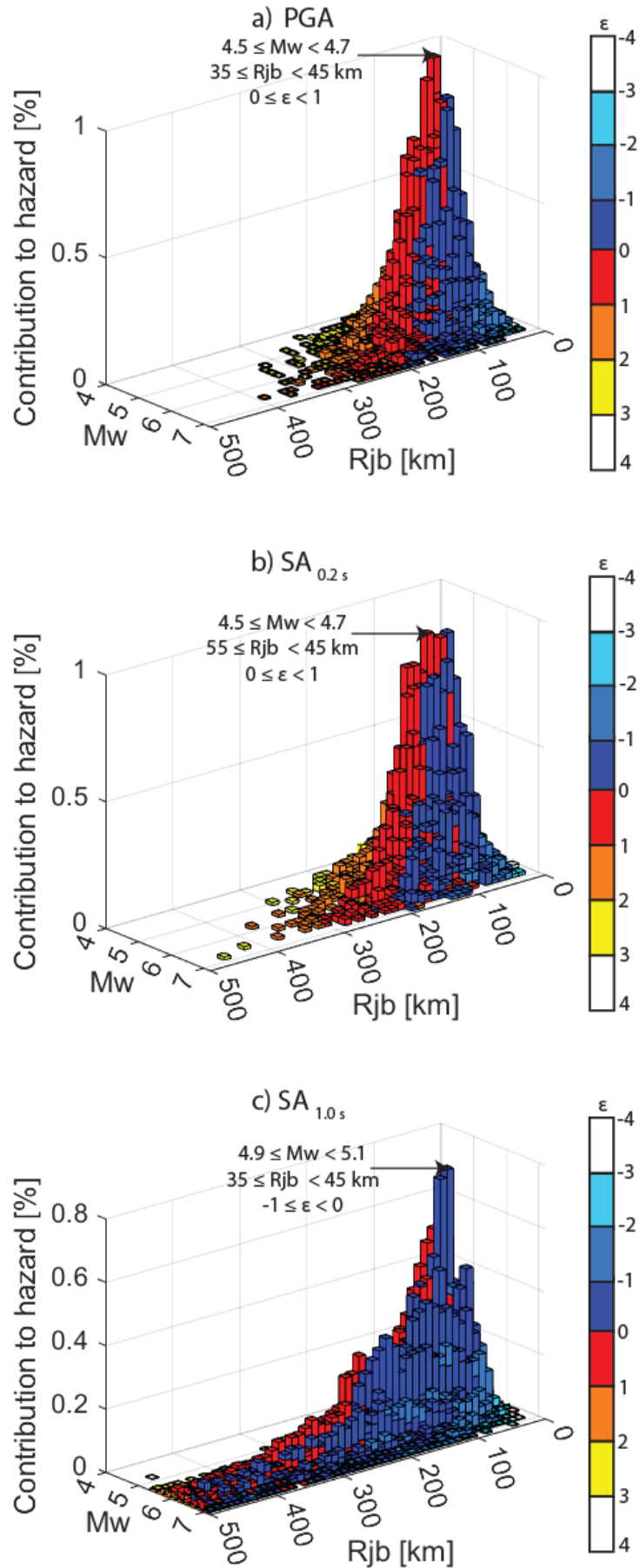
Figure 48: Disaggregation of the hazard for the HyNet site and 475-year return period by magnitude (Mw), Joyner-Boore distance (Rjb) and epsilon ( \epsilon ) for (a) PGA, (b) SA_{0.2s} , and (c) SA_{1.0s} .
