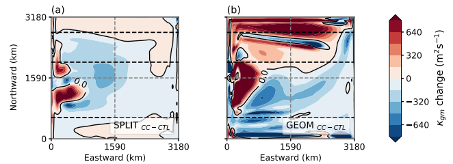
Fig. 8. Raw difference of the \kappa_{gm}(x, y) ( \text{m}^2 \text{s}^{-1} ) distribution between the climate change scenario and the control scenario (see Fig. 2) for (a) SPLIT, and (b) GEOM. The black dashed lines represent the sample latitudinal cross sections S_{1,2,3} going from south to north.
