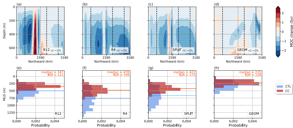
Fig. 9. (Top row) Raw difference of the meridional overturning streamfunction \Psi_{MOC} ( Sv = 10^6 m^3 s^{-1} ) between the climate change and the control scenario (Fig. 4a-d), for (a) R12, (b) R4, (c) SPLIT, and (d) GEOM; negative values largely indicate a weakening of the overturning strength. The black dashed lines represent the sample latitudinal cross sections S_{1,2,3} going from south to north. (Bottom row) The histogram of yearly maximum mixed layer depth distributions ( m , identified as the first depth below which |\sigma_\theta(z) - \sigma_\theta(z = -10 m)| > 0.01 where \sigma_\theta is the potential density referenced to sea level, with 20 bins ranging from 0–1500 m) and median (indicated by the horizontal line) over the area where deep water formation occurs, for the climate change scenario (in red) and control scenario (in blue, see Fig. 4e-h), for (e) R12, (f) R4, (g) SPLIT, and (h) GEOM; the median and inter-quartile range (IQR) is shown (in units of m ), and the axes of the histograms have been flipped for convenient visual comparison.
