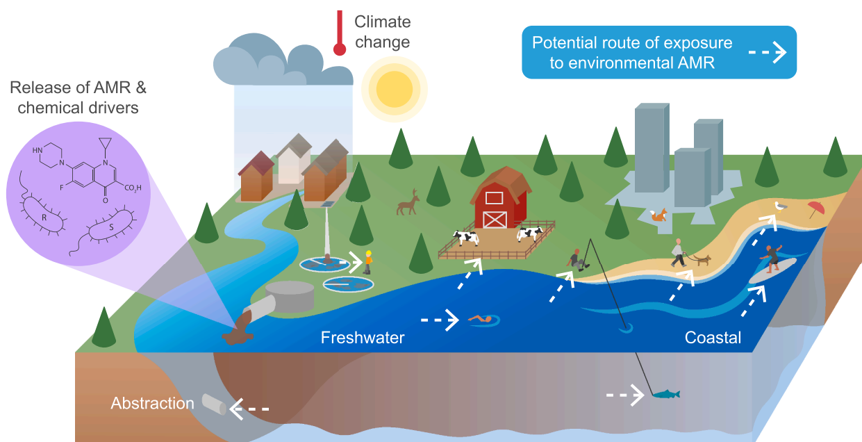
Fig. 1. Graphical overview of concepts discussed in the review. This highlights SO discharge of AMR and chemical drivers, potential exposure routes to humans of environmental AMR (indicated by white arrows), and future pressures, including increased rainfall and changes in temperature from climate change, and urbanisation.
