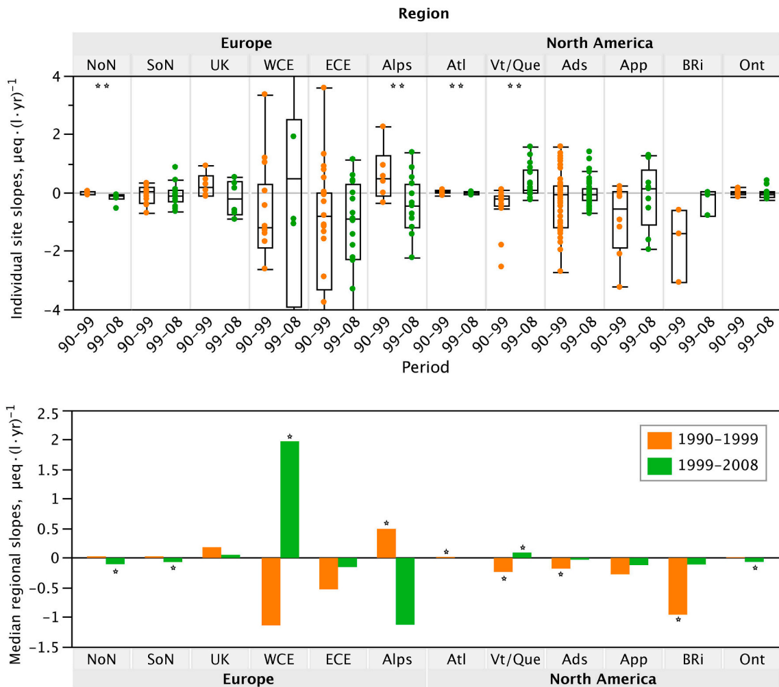
Fig. 28. Slopes of regional trends in concentrations of \text{NO}_3 for twelve regions in Europe and North America (North Nordic: NoN, South Nordic: SoN, United Kingdom: UK, West Central Europe: WCE, East Central Europe: ECE, Alps: Alps, Maine and Atlantic Canada: Atl, Vermont and Quebec: Vt/Que, Adirondacks: Ads, Appalachians: App, Blue Ridge Mountains: Bri and Ontario: Ont) for the time spans 1990-1999 and 1999-2008. The first figures indicate the individual site slopes with the boxes and whiskers covering the 25 th to 75 th and 10 th to 90 th percentiles of slopes, while the median is indicated in the second graph. Asterisks indicate the significance level (** p < 0.05 , * p < 0.10 ) of a non-parametric test for difference between the distributions of slopes for the two time periods. Source: Skjelkvåle and de Wit (2011) .
