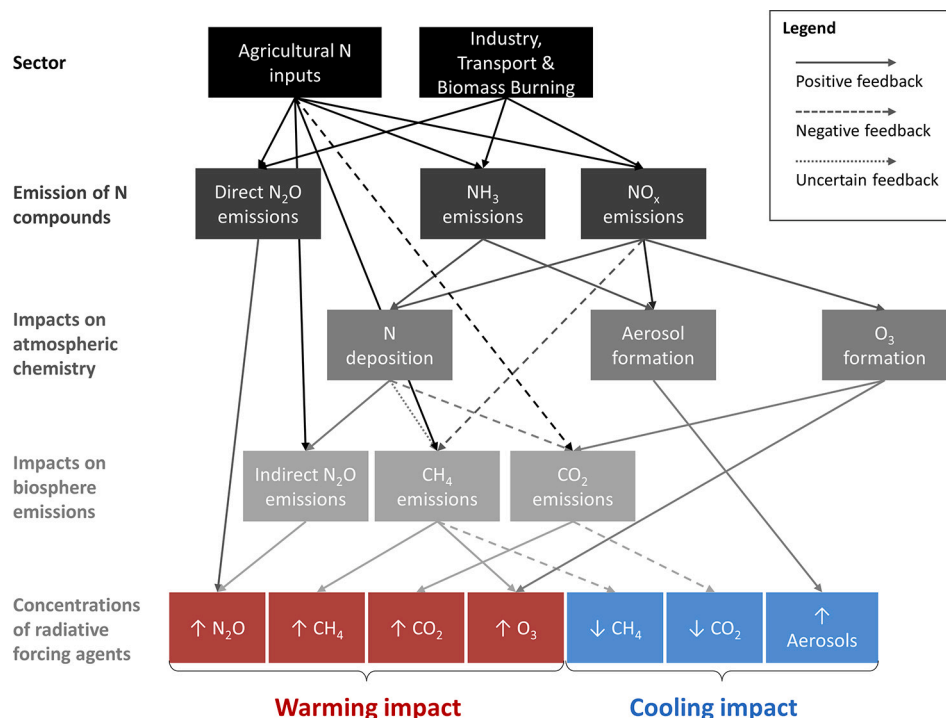
Fig. 11. Overview of impacts of intended and unintended reactive nitrogen production on radiative forcing (De Vries et al., 2023).
