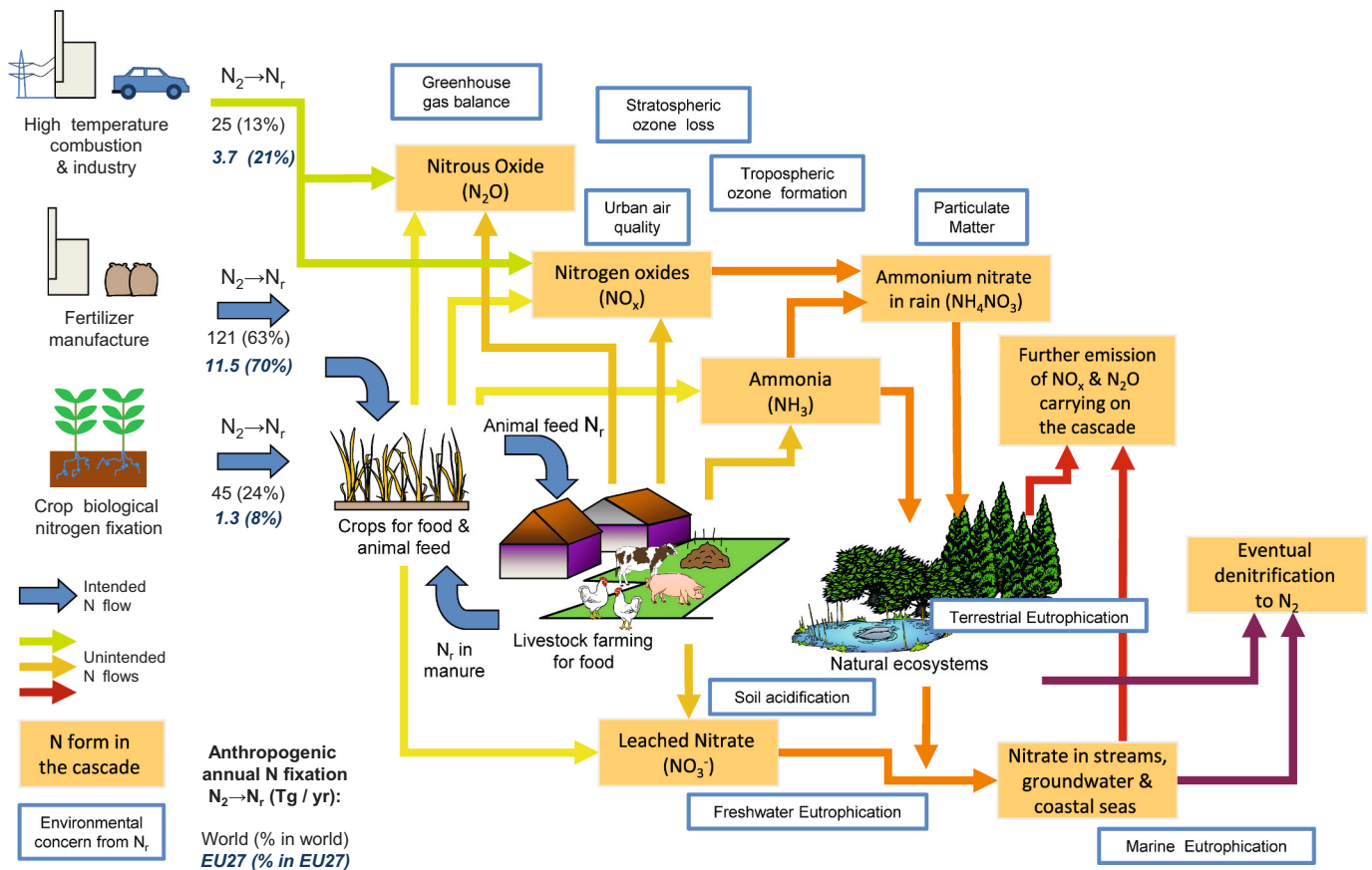
Fig. 1. Simplified view of the ‘Nitrogen Cascade’. At both European and global scales, the largest anthropogenic source of reactive nitrogen ( \text{N}_r ) enters agriculture via chemically fixed atmospheric \text{N}_2 and leaves agriculture in harvest products and via N losses to air ( \text{NH}_3 , \text{N}_2\text{O} and \text{NO}_x ), groundwater and surface waters ( \text{NO}_3^- , \text{NH}_4^+ , Dissolved Organic Nitrogen). Additional sources are biological N fixation and the inadvertent fixation of N through high-temperature combustion processes releasing \text{NO}_x in the industrial and transport sectors. \text{NO}_x emissions lead to ozone formation, and both \text{NO}_x and \text{NH}_3 contribute to particulate matter formation. These losses and their transformations create a sequence of ecological and human health effects, allowing one atom of fixed N to exert several different effects, with nine main threats illustrated here (based on Sutton et al., 2011a).
