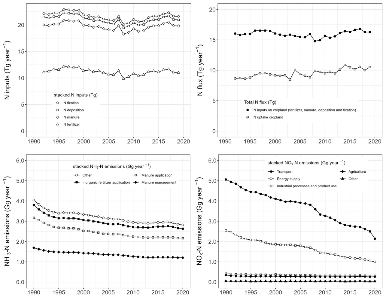
Fig. 2. Stacked nitrogen inputs to EU from 1990-2020 on cropland and fertilized grassland (top left), cropland N harvest (top right) and N inputs on cropland (top right) in \text{Tg N yr}^{-1} and stacked N emissions from both agriculture and other sources to air as \text{NH}_3 (bottom left) or \text{NO}_x (bottom right) in \text{Gg N yr}^{-1} . Data of N inputs and uptake are from Einarsson et al. (2021), the \text{NH}_3 and \text{NO}_x emissions to air from (EEA, 2023b). Note that the difference between total N inputs and N uptake in top left figure is the N surplus.
