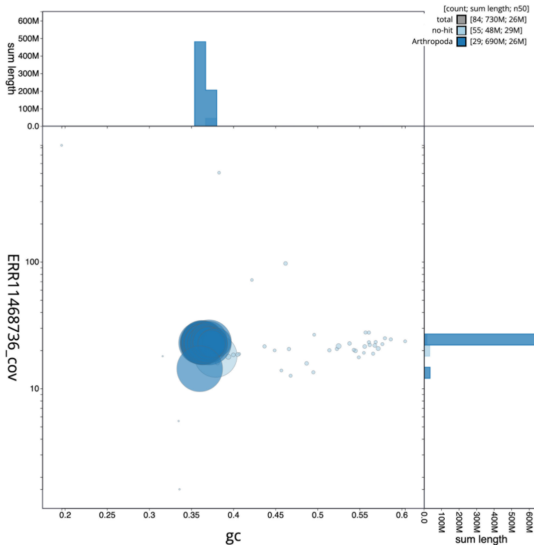
Figure 3. Genome assembly of Elophila nymphaeata , ilEloNymp1.1: BlobToolKit GC-coverage plot. Sequences are coloured by phylum. Circles are sized in proportion to sequence length. Histograms show the distribution of sequence length sum along each axis. An interactive version of this figure is available at https://blobtoolkit.genomehubs.org/view/ilEloNymp1_1/dataset/ilEloNymp1_1/blob .
