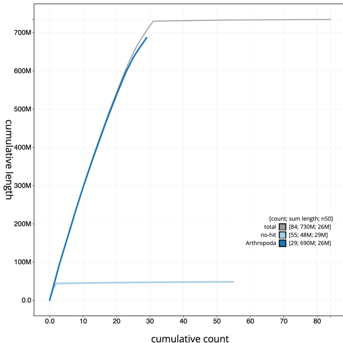
Figure 4. Genome assembly of Elophila nymphaeata , iEloNym1.1: BlobToolKit cumulative sequence plot. The grey line shows cumulative length for all sequences. Coloured lines show cumulative lengths of sequences assigned to each phylum using the buscogenes taxrule. An interactive version of this figure is available at https://blobtoolkit.genomehubs.org/view/iEloNym1_1/dataset/iEloNym1_1/cumulative .
