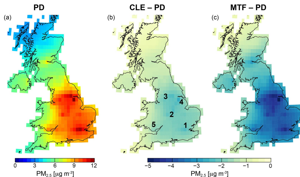
Figure 4. Effect of emission control measures on UK PM_{2.5} . Maps are GEOS-Chem annual mean PM_{2.5} in 2019 (PD) (a) and changes in PM_{2.5} relative to the PD due to controls on anthropogenic sources to meet current legislation (CLE minus PD) (b) and adoption of readily available maximum technically feasible measures (MTF minus PD) (c). Inset numbers in (b) are locations with greatest decline in PM_{2.5} discussed in the text: 1. London, 2. Birmingham, 3. Manchester and Leeds, 4. East Yorkshire, and 5. South coast of Wales.
