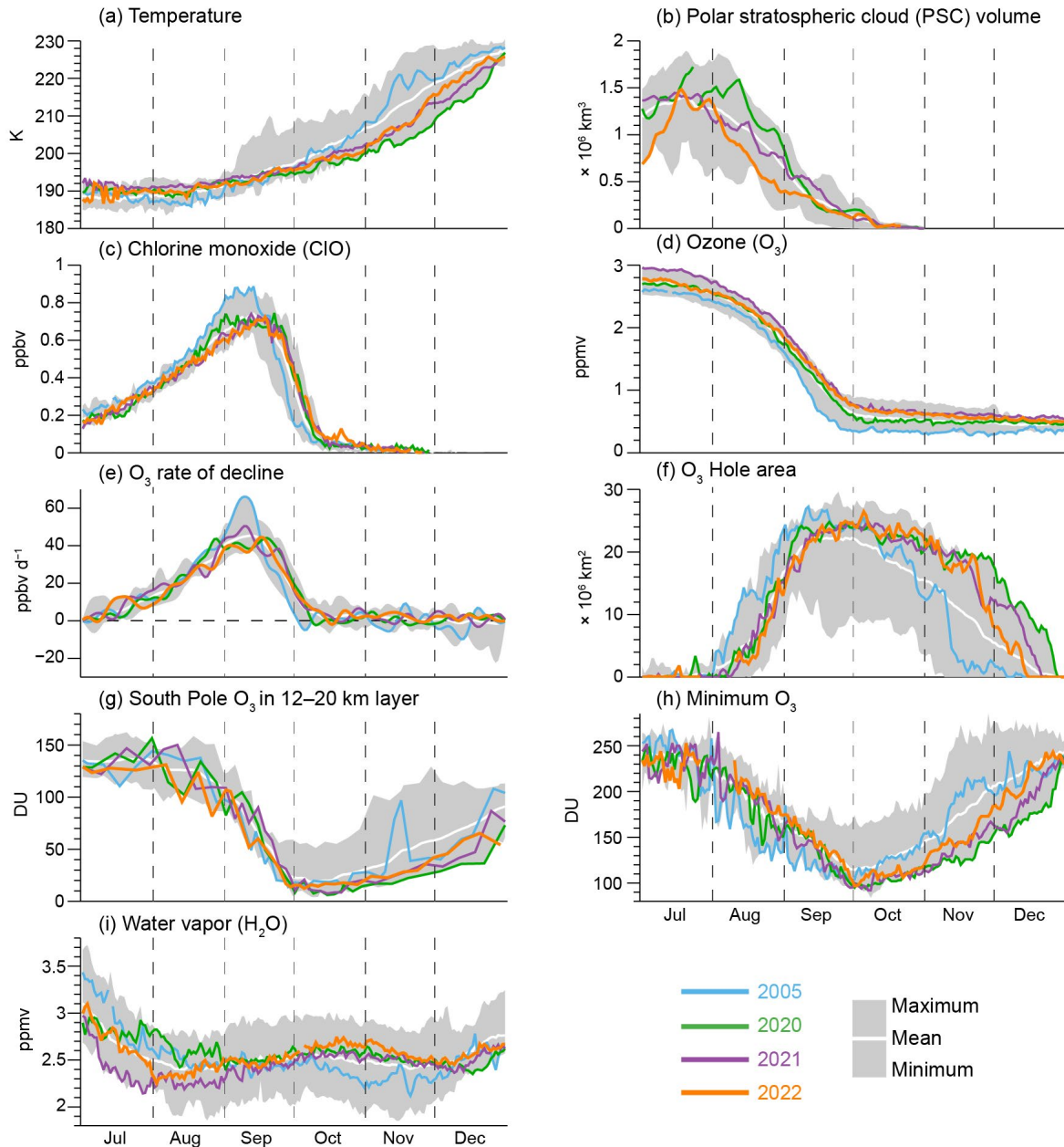
Fig. 6.15. Antarctic values of (a) vortex-averaged MERRA-2 temperature on the 440-K potential temperature surface (~19 km or 60 hPa), (b) CALIPSO polar stratospheric cloud (PSC) volume (updated from Pitts et al. 2018), (c),(d),(e),(i) vortex-averaged chlorine monoxide (ClO), ozone (O 3 ), O 3 rate of decline (calculated as time derivatives of vortex-averaged ozone), and water vapor (H 2 O) on the 440-K potential temperature surface from Aura MLS (updated from Manney et al. 2011), (f) OMI/OMPS Antarctic ozone hole area (area with ozone total column less than 220, DU), (g) lower stratospheric ozone columns (12 km–20 km) based on sonde measurements at South Pole, and (h) minimum total ozone columns over 60°S–90°S from OMI/OMPS. Gray shading shows the range of daily Antarctic values for 2005 (for all but (h), which starts in 2006) through 2021. The white curve indicates the 2005–21 long-term mean. DU is a unit of measurement of the amount of a trace gas in a vertical column. One DU represents the number of trace gas molecules in the 0.01-mm-thick layer at standard atmospheric surface conditions.
