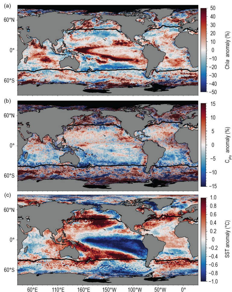
Fig. 3.25. Spatial distribution of average monthly (a) MODIS-A chlorophyll-a (Chl a ) anomalies (%), (b) MODIS-A phytoplankton carbon (C phy ) anomalies (%), and (c) MODIS-A sea-surface temperature (SST) anomalies (°C) for Oct 2021–Sep 2022, where monthly differences were derived relative to the MODIS-A 19-year climatological record (Oct 2002–Sep 2021). Chl a and C phy are stated as % difference from climatology, while SST is shown as an absolute difference. Also shown in each panel is the location of the mean 15°C SST isotherm (black lines) delineating the permanently stratified ocean. Differences in the SST anomalies here versus in Fig. 3.1 are owing to differences in climatological periods, smoothing, and data sources.
