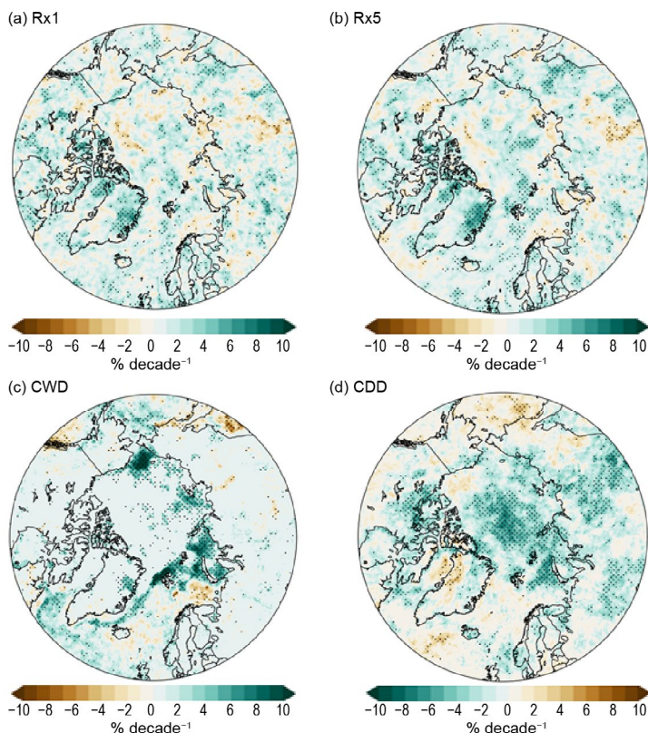
Fig. 5.7. Trends of daily extreme precipitation indices (% decade -1 ) over the period 1950–2021. Plots are shown for yearly maximum one-day total precipitation (Rx1; upper left), yearly maximum five-day amount (Rx5; upper right), yearly maximum number of consecutive wet days (CWD; lower left), and yearly maximum number of consecutive dry days (CDD; lower right). Green shades denote trends toward wetter extremes; brown shades denote trends towards drier extremes. Stippling denotes trend significance at the 0.05 level. (Source: ERA5.)
