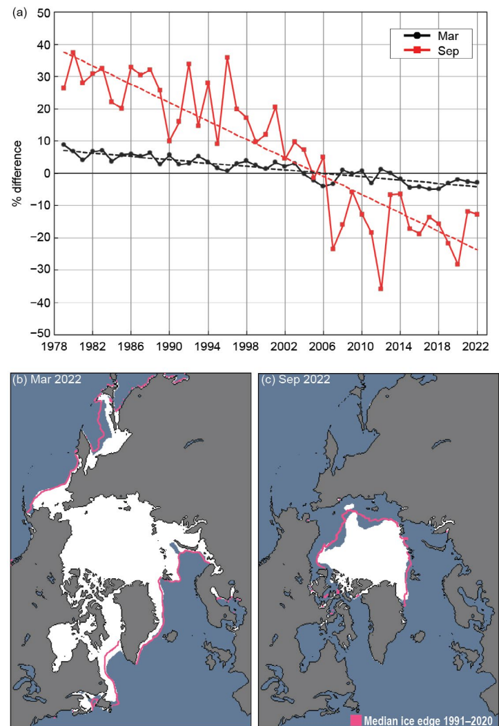
Fig. 5.11. (a) Monthly sea-ice extent anomalies (%), solid lines) and linear trend lines (dashed lines) for Mar (black) and Sep (red) from 1979 to 2022. The anomalies are relative to the 1991–2020 average for each month. (b) Mar 2022 and (c) Sep 2022 monthly average sea-ice extent; the median extent for 1991–2020 is shown by the magenta contour.
