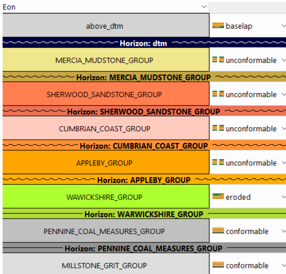
Figure 8 Stratigraphy and unconformities used in the SKUA-GOCAD Bedrock model. BGS © UKRI 2023.
