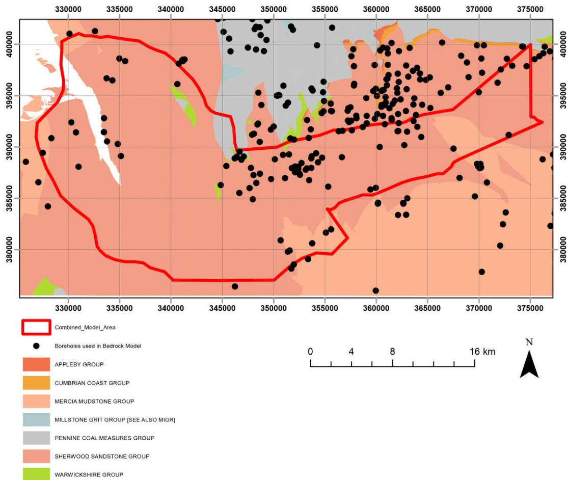
Figure 7 Locations of the boreholes used to inform the bedrock model. BGS © UKRI 2023.
