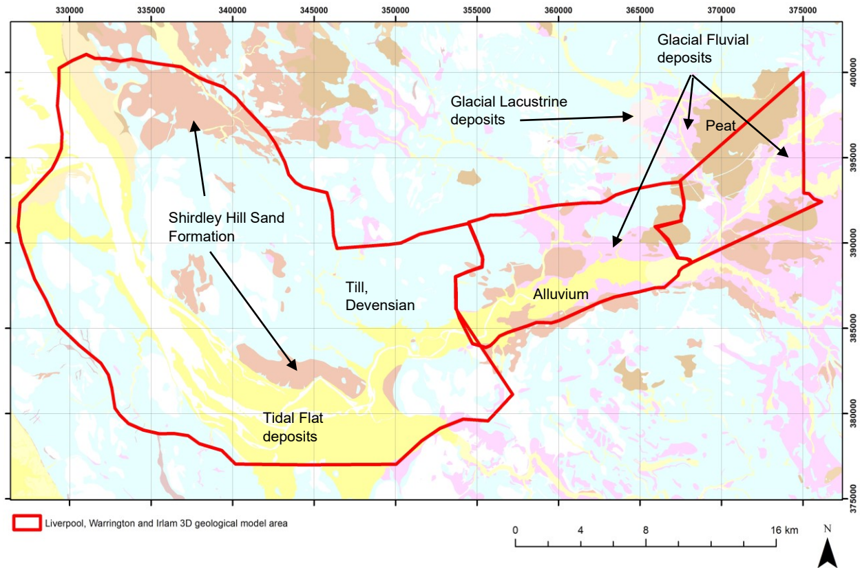
Figure 3 BGS Superficial deposits 50k - 3D geological model area. BGS © UKRI 2023.
