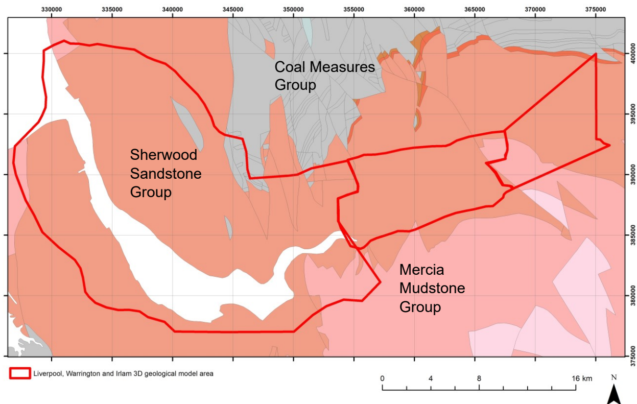
Figure 2 BGS Geology 250k – 3D geological model area. BGS © UKRI 2023.
