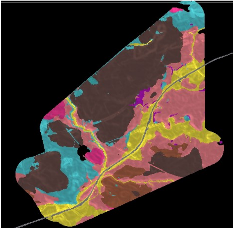
Figure 12 3D view of the Irlam area from above, showing superficial deposits and artificially modified ground, vertical exaggeration x10. Legend as per Table 1. BGS © UKRI 2023.
