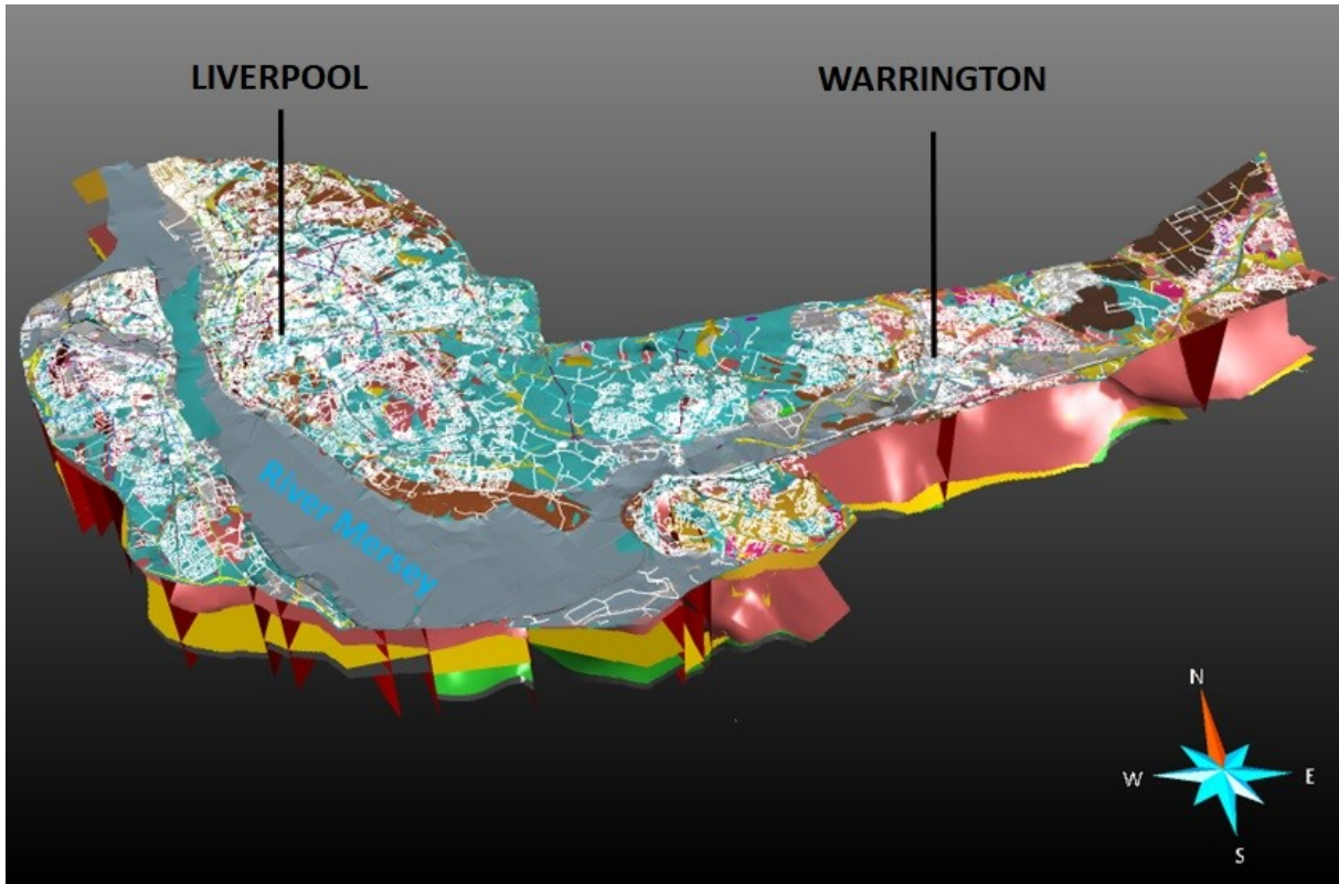
Figure 9 3D view of the combined superficial and bedrock model with 10x vertical exaggeration. Legend as per Table 1. BGS © UKRI 2023.
