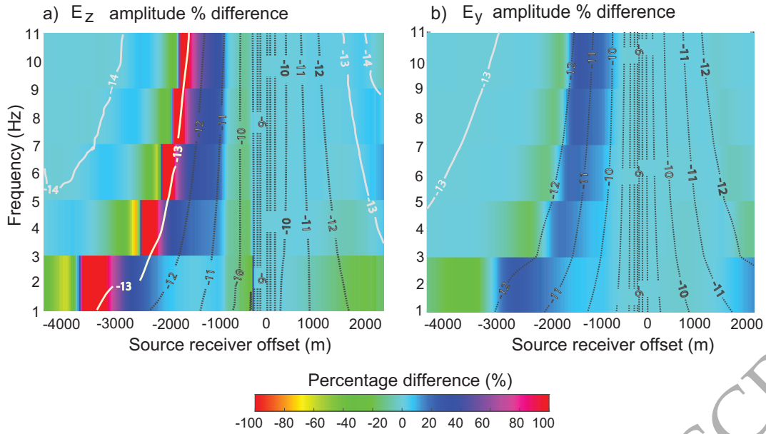
Figure 8. Amplitude percentage difference between chimney saturated with 20 per cent CO 2 (model in Figure 3d) and a chimney saturated with brine or S CO 2 =0 (model in Figure 3b) for E z a) and E y b). This amplitude anomaly in percentage difference for the 2D model with S CO 2 =20 per cent is calculated for a receiver 1000 m away from the chimney (OBE-D). Dashed black contours correspond to the log 10 electric field amplitude of the model saturated with 20 per cent CO 2 . STEMM-CCS survey instrument noise floor at 10 -13 V/Am 2 , contours below noise floor marked with a continuous white line. Color represents the percentage difference.
