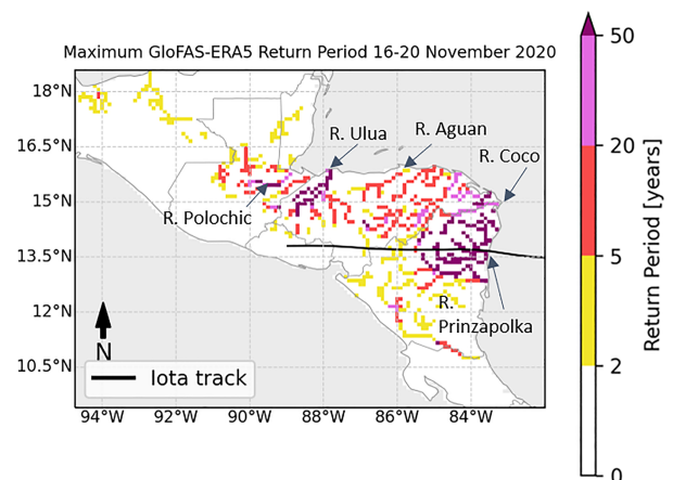
FIGURE 2 Iota maximum GloFAS-ERA5 return period 16th–20th November 2020. The purple colours indicate the expected locations of the most severe inland flooding. Labels identify major river of interest.
