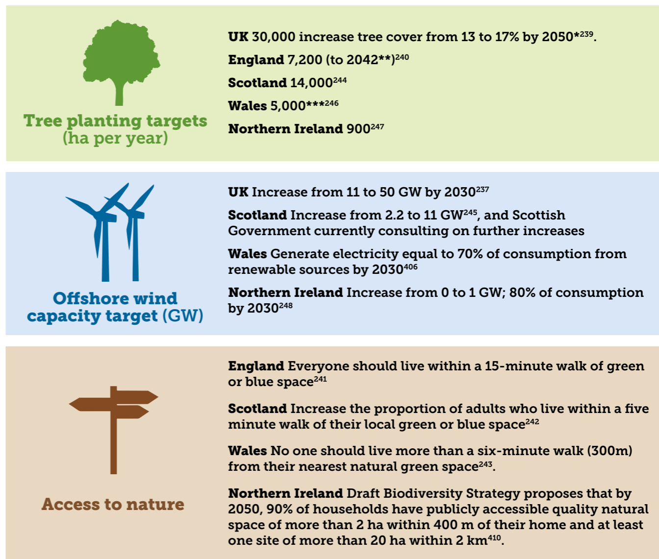
Figure 22: Targets for tree planting, offshore wind energy capacity and people's access to nature, for the UK and UK countries. Not all countries have a target in each area.
