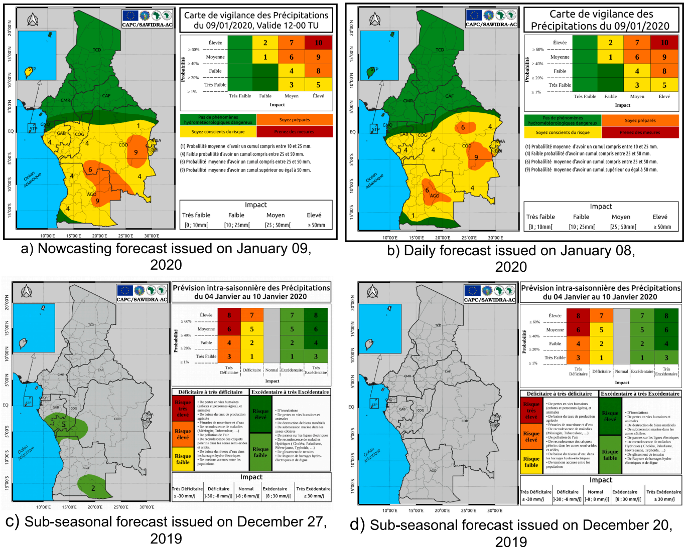
Fig. 3. Forecast bulletins valid for 09 January 2020 issued on (a) 09 January 2020, (b) 08 January 2020, (c) 27 December 2019 and (d) 20 December 2019.
