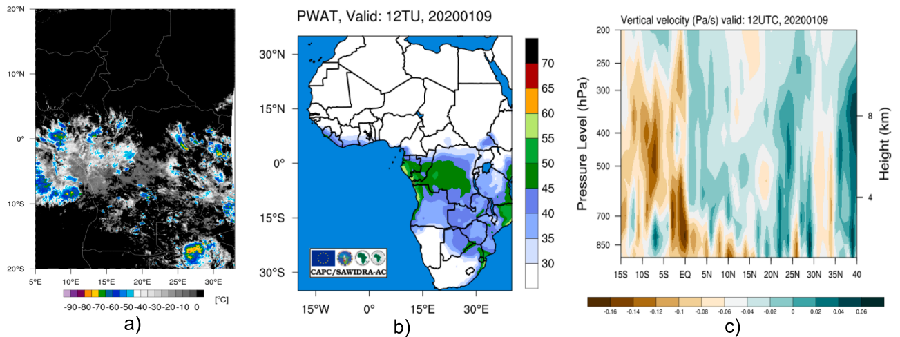
Fig. 5. Selected products used for nowcasting on 9th January 2020 including: a) EUMETSAT IR10.8 image (°C) at 11 UTC 9th January 2020; b) GEFS precipitable water forecast (mm); and c) GEFS vertical velocity ( \text{Pa s}^{-1} ).
