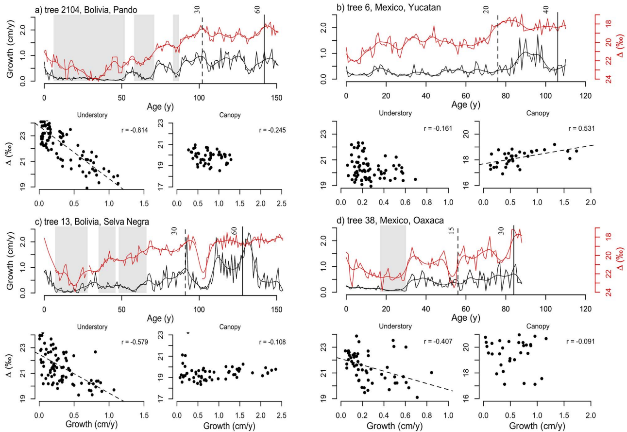
Figure 4. Examples of trajectories for growth (black lines) and C-isotope discrimination ( \Delta^{13}\text{C} , red lines in reversed axes) of individual trees, and scatterplots of growth versus \Delta^{13}\text{C} for understory and canopy growth phases. Note the reverse axis for \Delta^{13}\text{C} time series in red in the upper panels. Understory is defined as trees smaller than 30, 20 and 15 cm in diameter for Bolivia, Yucatan and Oaxaca, respectively, which is the approximate size at which trees reach the lower canopy (see Materials and methods). The age at which the individual trees reached these diameter thresholds for understory versus canopy growth phases or larger canopy sizes are indicated in the trajectory plots with vertical broken and continuous lines, respectively, with numbers referring to tree diameter in cm. The trend lines in the scatter plots indicate significant ( P < 0.05 ) relationships between early growth rate and \Delta^{13}\text{C} , and Pearson correlation coefficients ( r ) are shown. Smooth curves for growth and \Delta^{13}\text{C} trajectories are smoothing splines (see Materials and methods). Periods of suppression (i.e., minimum of 5 years of growth below a site-specific threshold, see Materials and methods) are indicated by shaded areas.
