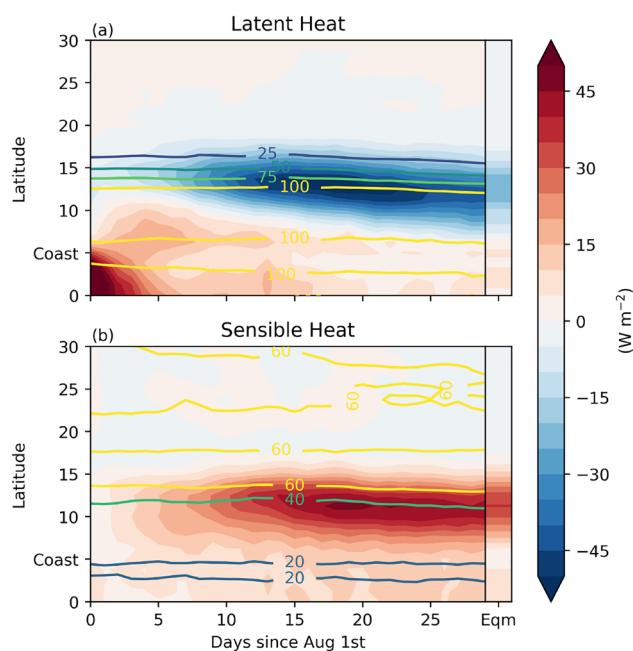
Fig. 12 HadGEM2-A (left of vertical black line) climatological (amip) (lines) and spin-up anomalous (amip-p4K-spinup - amip) (shaded colors) and (right of vertical black line) August equilibrium anomalous (amip-p4K - amip); a latent heat flux, and b sensible heat flux
