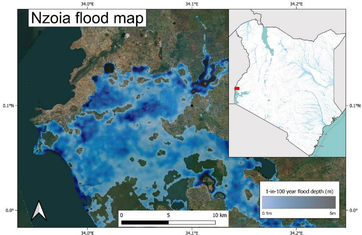
FIGURE 9 1-in-100-year return period flood map for Nzoia, Kenya derived using the Fathom GFM model under the SHEAR HyPac project
