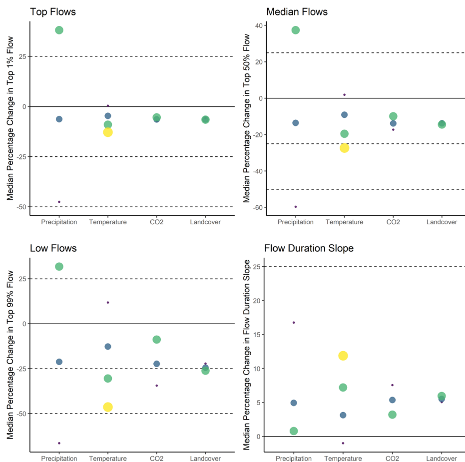
360 Figure 6: Median percentage change in the indicated four metrics for catchments based on precipitation, temperature, CO 2 , and afforestation changes. Increasing dot size and lighter colour indicate larger changes in the variables explored (precipitation: 70%, 100%, 130%; temperature: 0 °C, +1 °C, +2 °C, +3 °C; CO 2 : 375 ppm, 425 ppm, 600 ppm; afforestation: 0%, 50%, 100%). Colours are used to further differentiate variable quantity and are not relative to the size of the variable. The solid black horizontal line indicates a 0 % change for all variables whereas the dashed lines indicate defined intervals of change.
