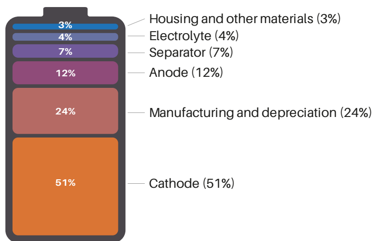
Figure 19 The estimated cost breakdown of a lithium-ion battery cell. Data source: Bloomberg (2021).
