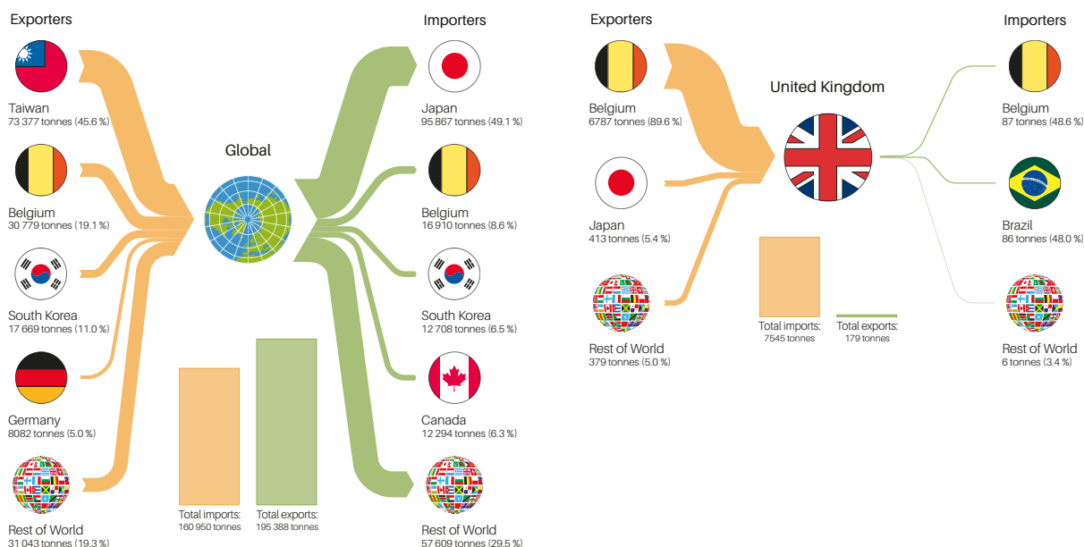
Figure 24 Global and UK trade of sulphates of nickel in 2019. Data source: DESA/UNSD (2022), United Nations Comtrade database; HS code: 283324; Taiwan = Other Asia, nes; South Korea = Rep. of Korea.
