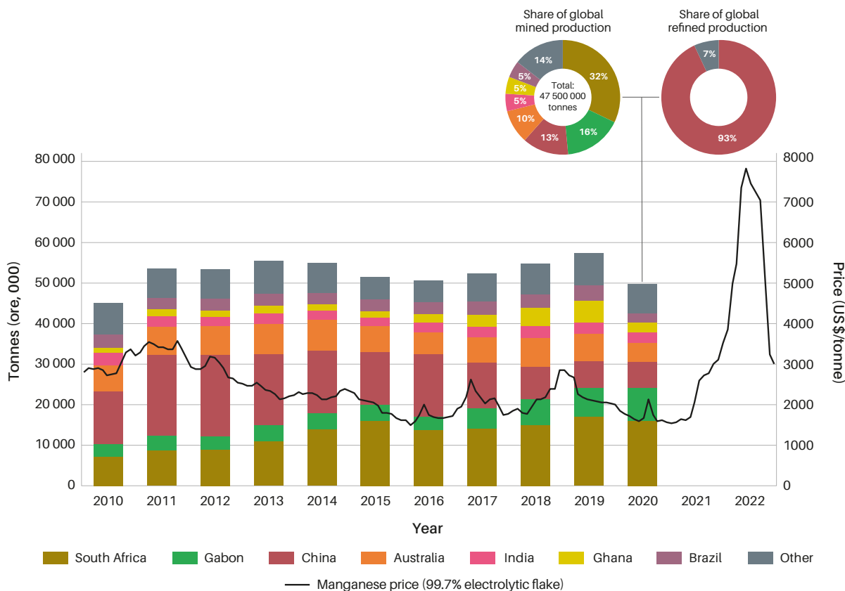
Figure 17 Global production of manganese between 2010–2020, data source: British Geological Survey (2022) and the price of manganese (99.7 per cent electrolytic flake) from 2010–May 2022, data source: Fastmarkets (2022).
