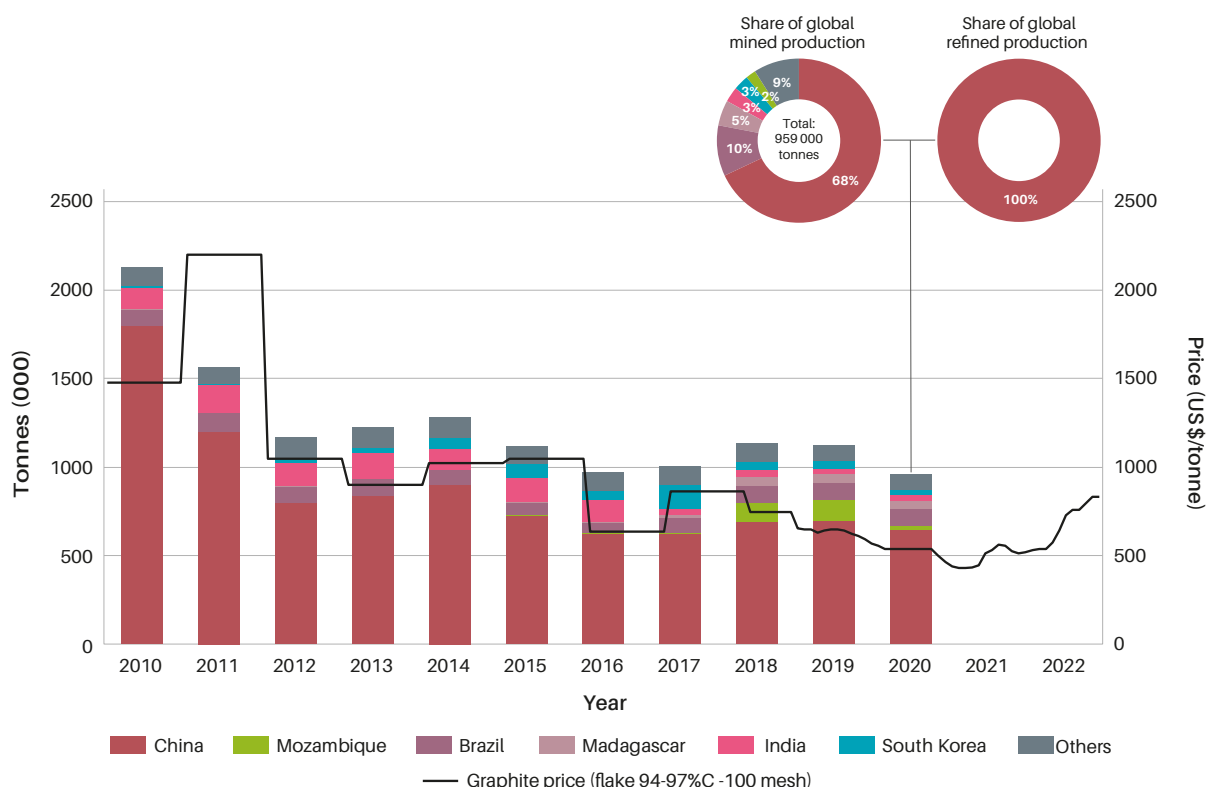
Figure 18 Global production of natural graphite between 2010–2020, data source: British Geological Survey (2022) and the price of graphite (flake 94–97 per cent, -100 mesh) from 2010–May 2022. Annual price data from 2010–2018, data source: USGS, 2022, and monthly price data from August 2018–May 2022, data source: Fastmarkets (2022).
