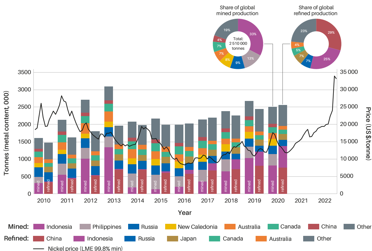
Figure 15 Global production of mined and refined nickel between 2010–2020, data source: British Geological Survey (2022) and the price of nickel metal (LME 99.8% minimum) from 2010–May 2022, data source: Fastmarkets (2022).
