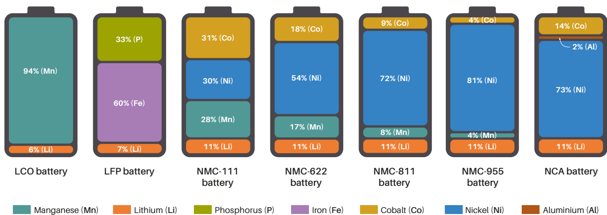
Figure 3 Key lithium-ion battery types and their key cathode constituents. Adapted from Gunn and Petavratzi (2018) and BloombergNEF (2020). BGS © UKRI.
