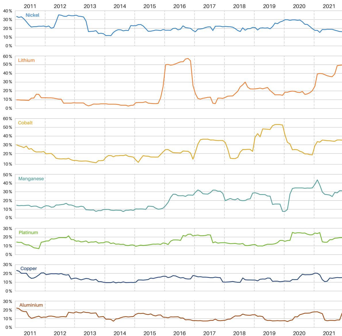
Figure 20 Monthly price volatility for the battery minerals and selected other metals for comparison (platinum, copper, aluminium). Prior to August 2018 only annual data is available for graphite. Data source: Fastmarkets (2022).
