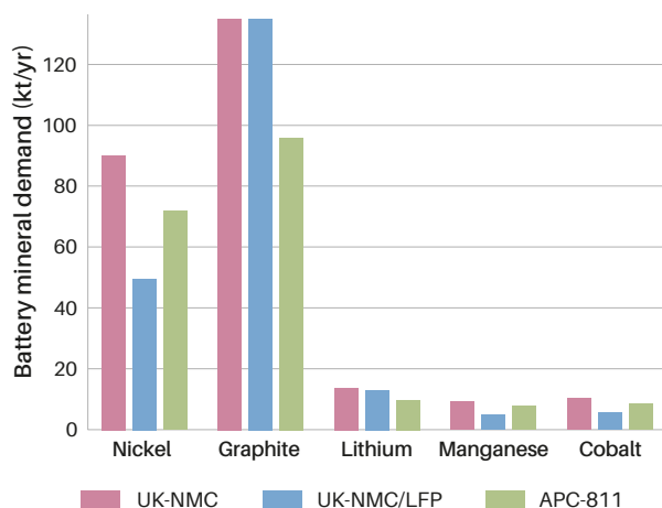
Figure 6 Estimated annual UK demand (kt = thousand tonnes) for battery minerals in 2030 based on the announced capacity of UK gigafactories (Table 3 and Table 5), under two scenarios: i) the UK-NMC scenario is based on the various battery chemistries that the announced UK gigafactories plan to produce; and ii) the UK-NMC/LFP scenario assumes that 50 per cent of the announced UK capacity is used to make LFP batteries. The third demand assessment (APC-NMC-811) is based on forecasts of UK light duty electric vehicle production and assumes all cells use NMC-811 (Advanced Propulsion Centre, 2022a). BGS © UKRI.
