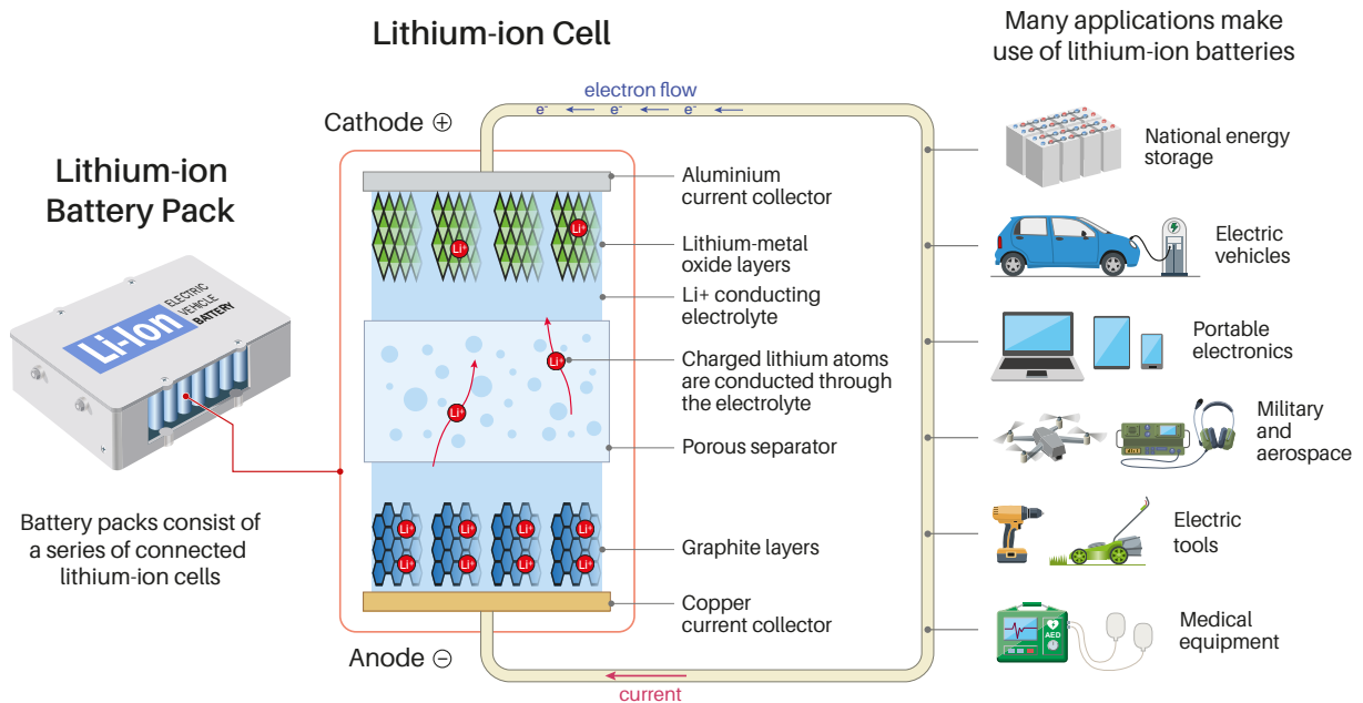
Figure 2 Schematic diagram of a lithium-ion battery and example end-use applications. During discharge, the anode releases free lithium ions to the cathode, providing an equal number of electrons to the electrical circuit. As a lithium-ion battery is being recharged, electric power imbalances the redox equilibrium between the anode and cathode, forcing the lithium ions to migrate back to the anode. BGS © UKRI.
