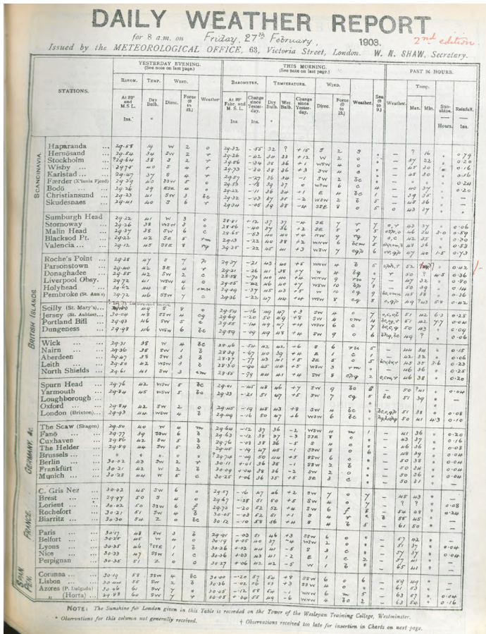
Figure A1. The UK Daily Weather Report observations page for 27 February 1903 (left; from NMLA, 2023) and tide gauge measurements from Liverpool Docks for 26–27 February 1903 (right; supplied by authors).
