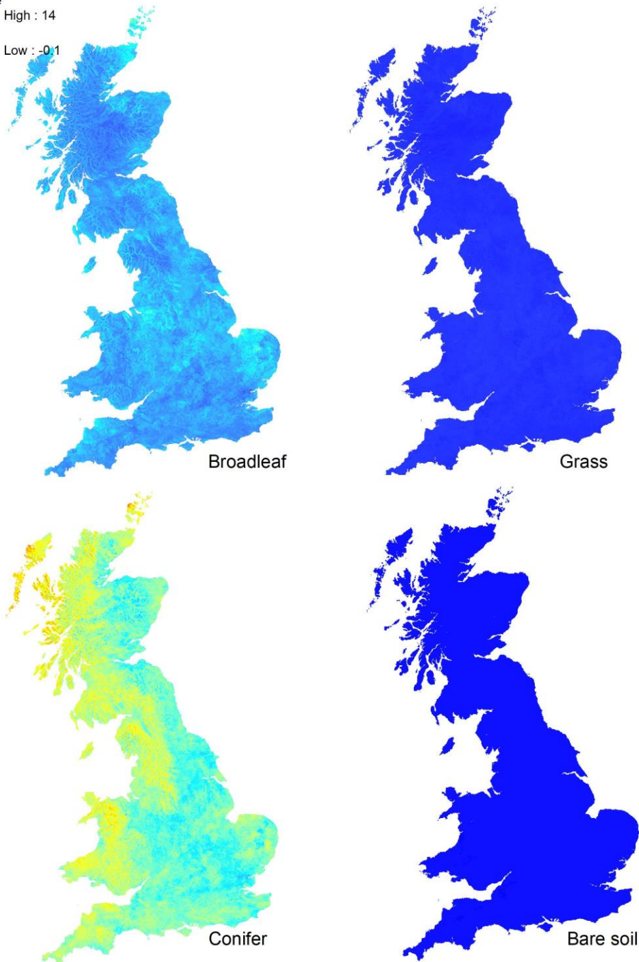
Figure 4 Spatial variation in mean daily interception loss on days with >25 mm rainfall (2005-2016) for the four land covers.
