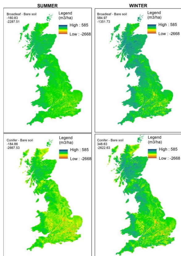
Figure 6 Calculated seasonal potential below ground flood storage in m 3 /ha to 3 m depth under broadleaf and conifer compared to (a) bare soil and (b) grass (2005-2016).
