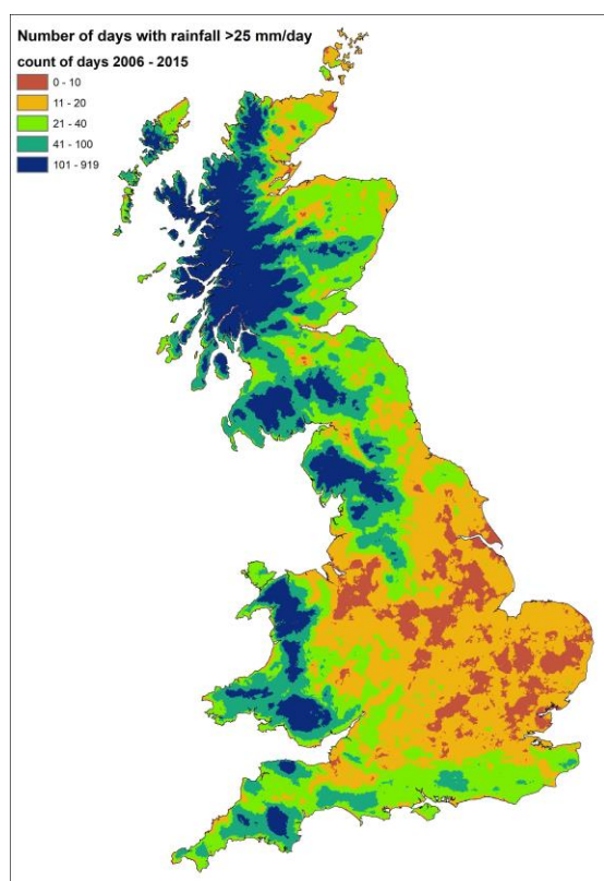
Figure 3 Number of days (2006 – 2015) with rainfall >25 mm used to estimate storm day interception loss for potential flood events.
