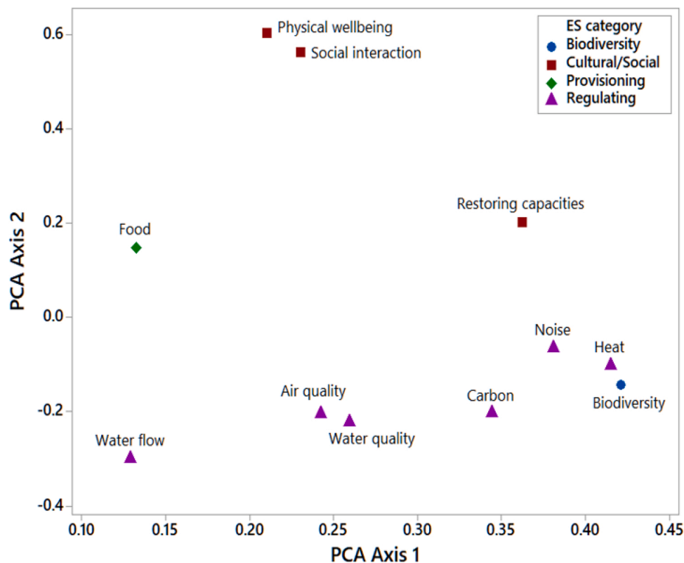
Fig. 3. Relationships amongst ecosystem services (ES), by principal components analysis. For interpretation of axes see Fig. 2.
