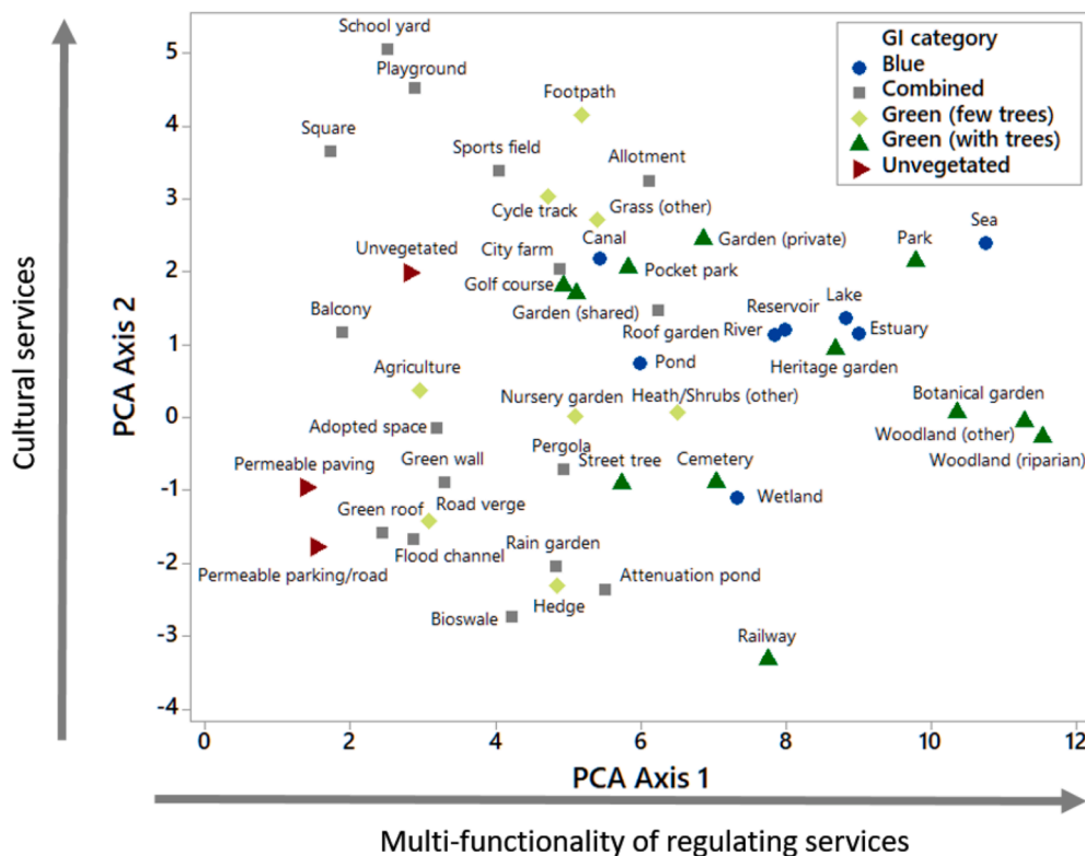
Fig. 2. Principal components analysis showing relationships amongst GI types. Axis 1 represents increasing naturalness and multi-functionality of regulating ecosystem services, while axis 2 represents increasing potential to support cultural services. ‘Combined’ features (grey squares) have a large constructed element as well as green or blue elements.
