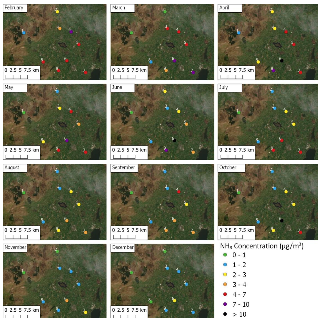
Figure 8: Monthly NH 3 concentration at measurement sites around Ballynahone Bog in 2019.
