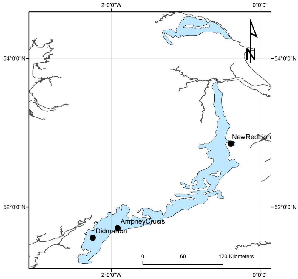
Figure 1. Extent of the Jurassic aquifer and borehole locations. Contains Ordnance Survey data © Crown copyright and database right [2022]
