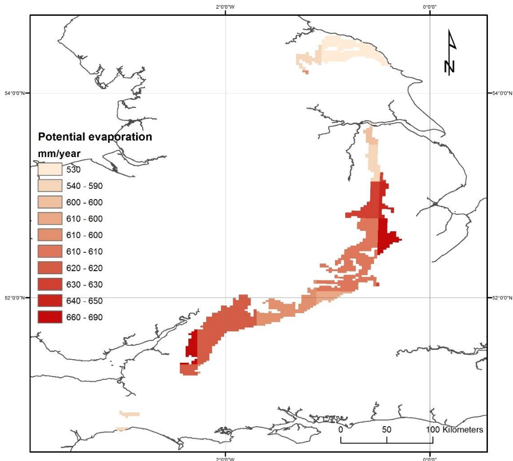
Figure 5. Spatial distribution of potential evaporation in the Jurassic aquifer. Contains Ordnance Survey data © Crown copyright and database right [2022]
