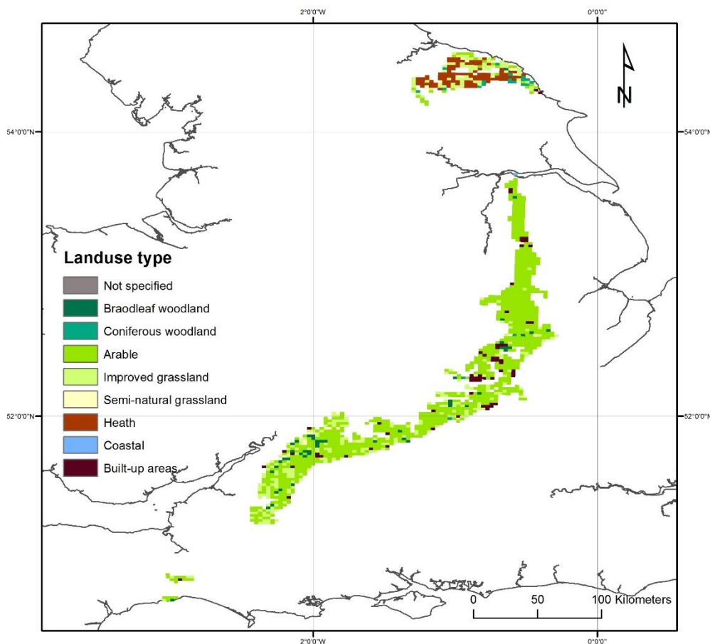
Figure 3. Map of land use over the Jurassic formation. Contains Ordnance Survey data © Crown copyright and database right [2022]
