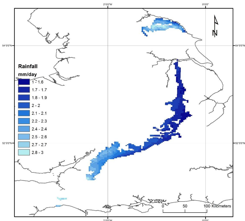
Figure 4. Spatial distribution of rainfall in the Jurassic aquifer. Contains Ordnance Survey data © Crown copyright and database right [2022]
