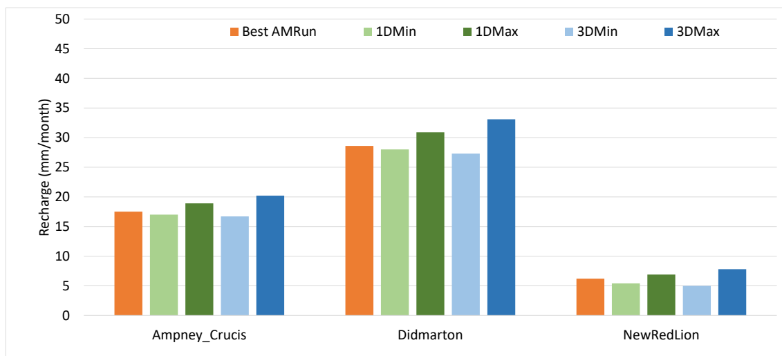
Figure 11 Historical (orange) and future recharge values (blue and green) as produced by the best performing AquMod model.
