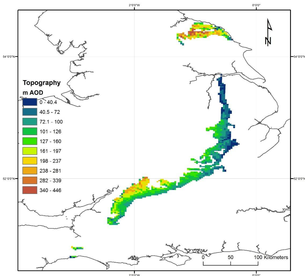
Figure 2. Topography map over the Jurassic formation. Contains Ordnance Survey data © Crown copyright and database right [2022]
