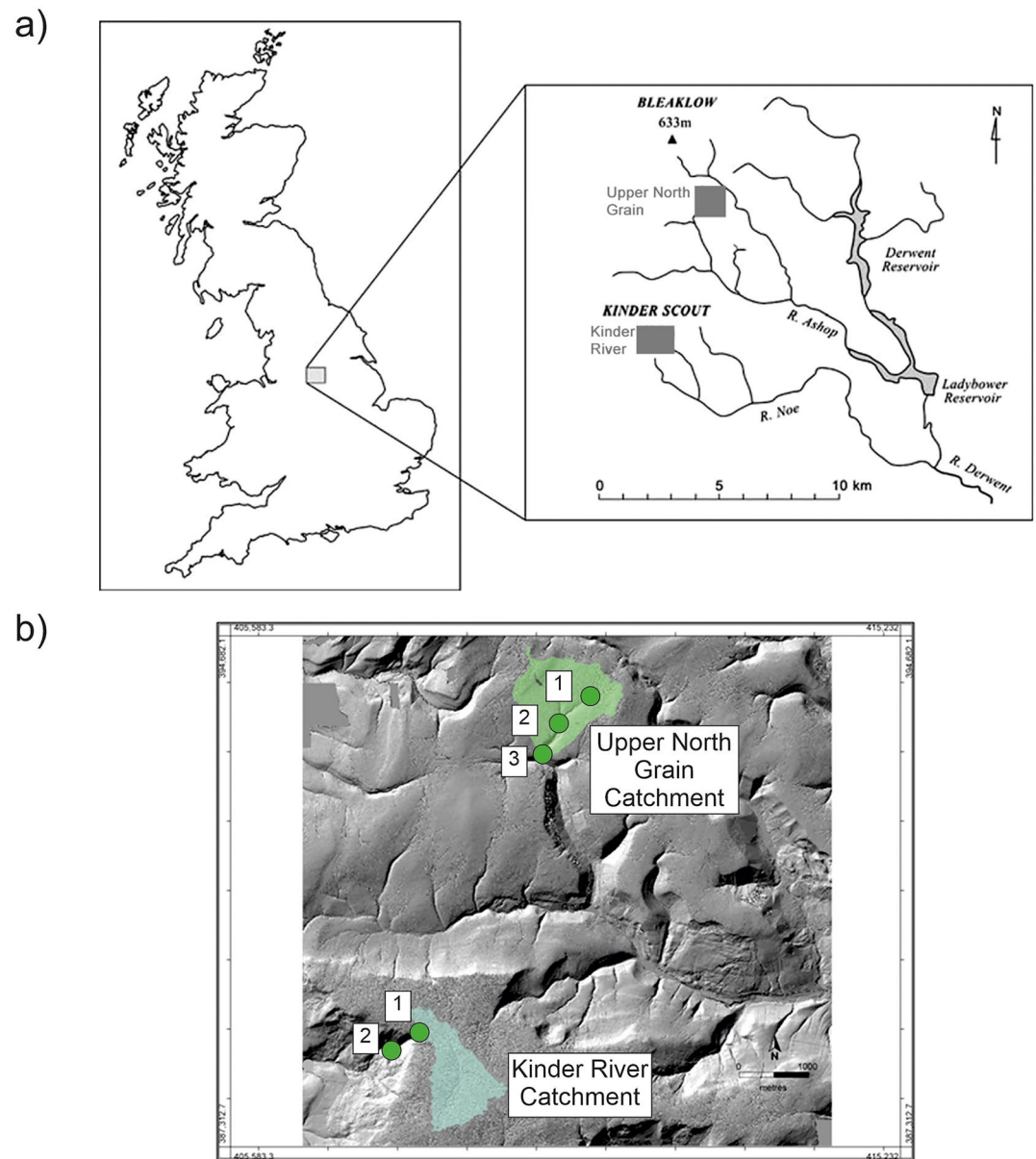
Figure 2. Study sites location and sampling points. (a) Location of Bleaklow Plateau and Kinder Scout in relation to the UK and each other. (b) Hillshade digital elevation model identifying the two study catchments and green dots representing the location of the sampling points.
