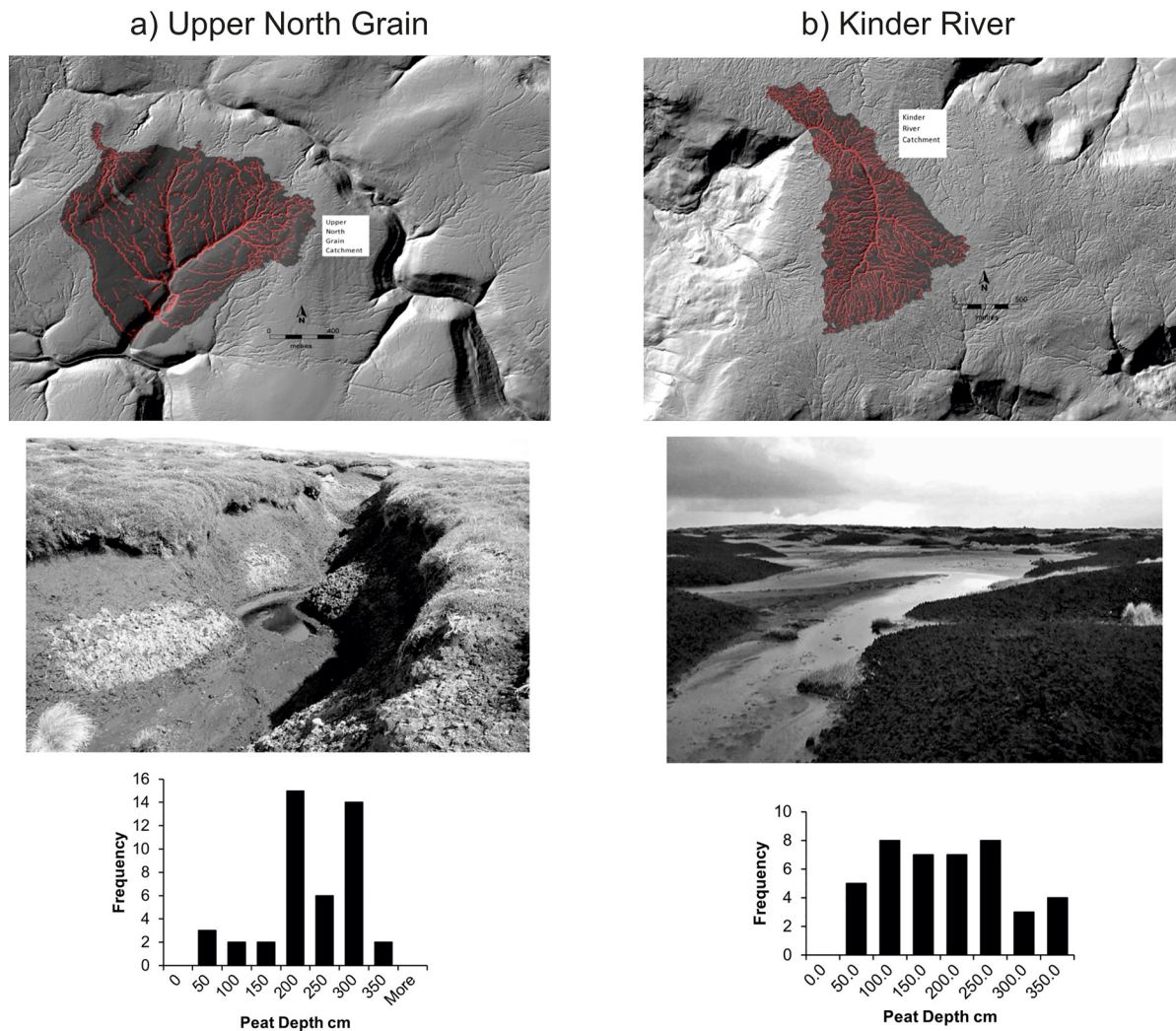
Figure 3. Hillshade Digital Elevation Model of study catchments with the gully network highlighted. Photos of the nature of erosion and peat depth distributions. (a) Gully erosion in the Upper North Grain (UNG) catchment. (b) Extensive bare peat and sheet erosion in the Kinder River catchment.
