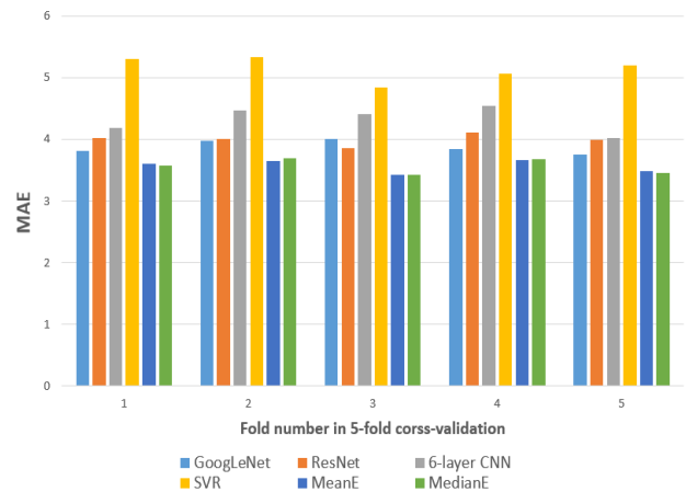
Fig. 4. Performance of each individual model.
