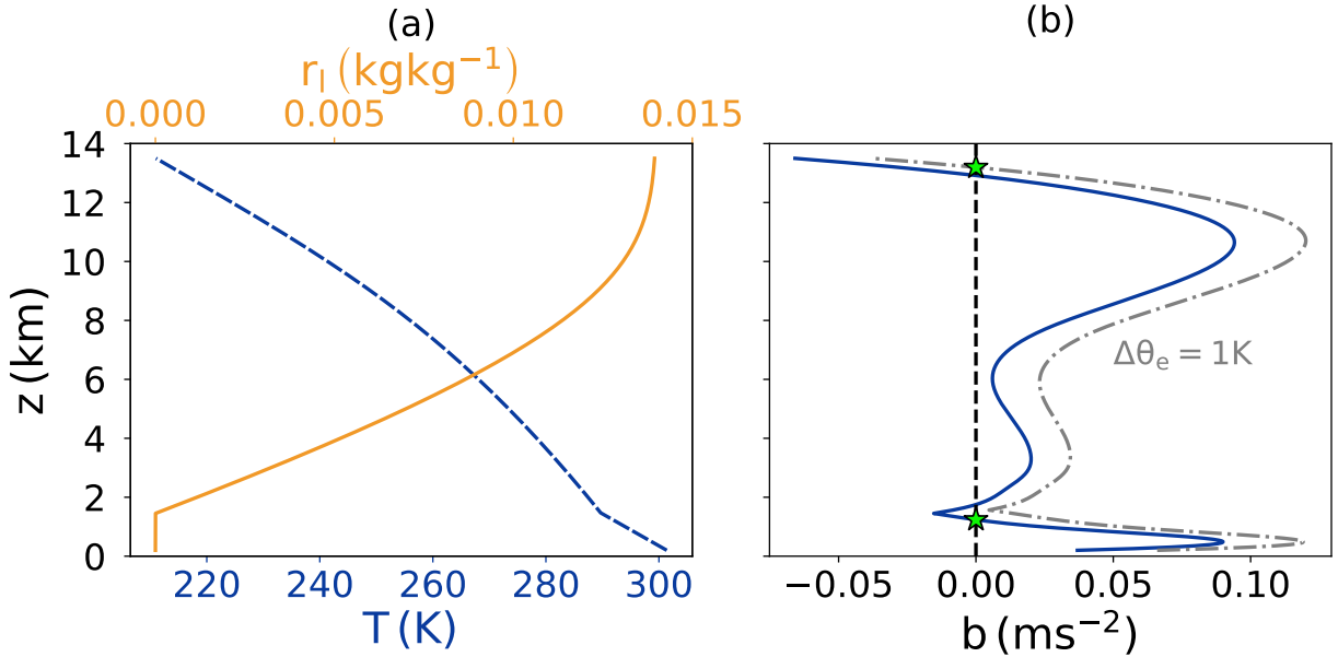
FIG. 3: Thermodynamic properties of a parcel with \theta_e = 340\text{ K} , r_l = 0.014\text{ kg kg}^{-1} when lifted reversibly and adiabatically upwards from 200 m through the Jordan hurricane-season mean sounding (freezing not included). (a) Temperature (dashed blue line) and liquid water mixing ratio (solid orange line) as parcel is lifted. (b) Buoyancy relative to Jordan sounding during lifting (blue solid line). The grey dashed-dotted line shows the buoyancy profile when \theta_e is perturbed by 1 K. The black dashed line indicates where b = 0\text{ m s}^{-2} . Green stars mark reference heights for the two parcels.
