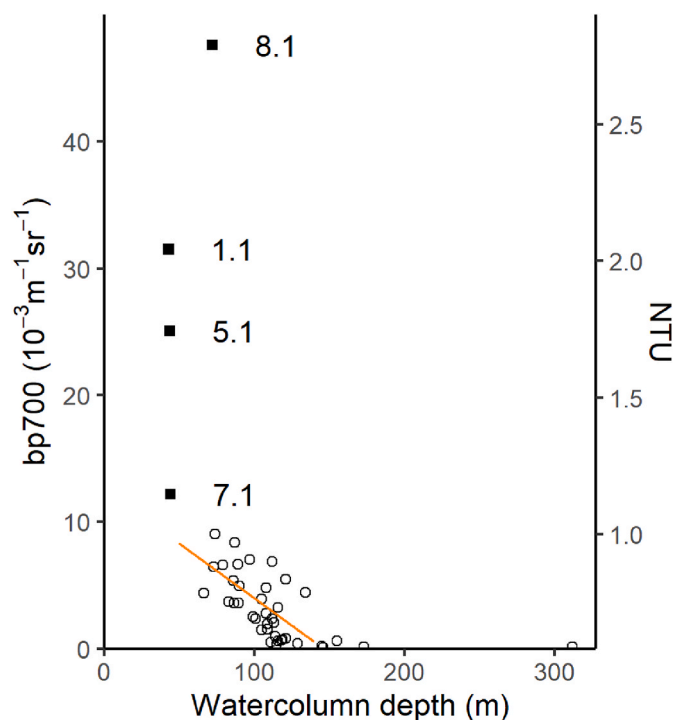
Fig. 9. Correlation between backscatter strength (mean of bp700 in 10^{-3} \text{m}^{-1} \text{sr}^{-1} 5 m above the seabed) and water column depth (in m). Solid squares show high concentrations at station 1.1, 5.1, 7.1 and 8.1. Orange line shows linear regression of all stations except the deep station (>300 m) and stations 1.1, 5.1 and 8.1 ( p < 0.001 , R^2 = 0.54 , n = 39 ). Corresponding NTUs are also shown.
