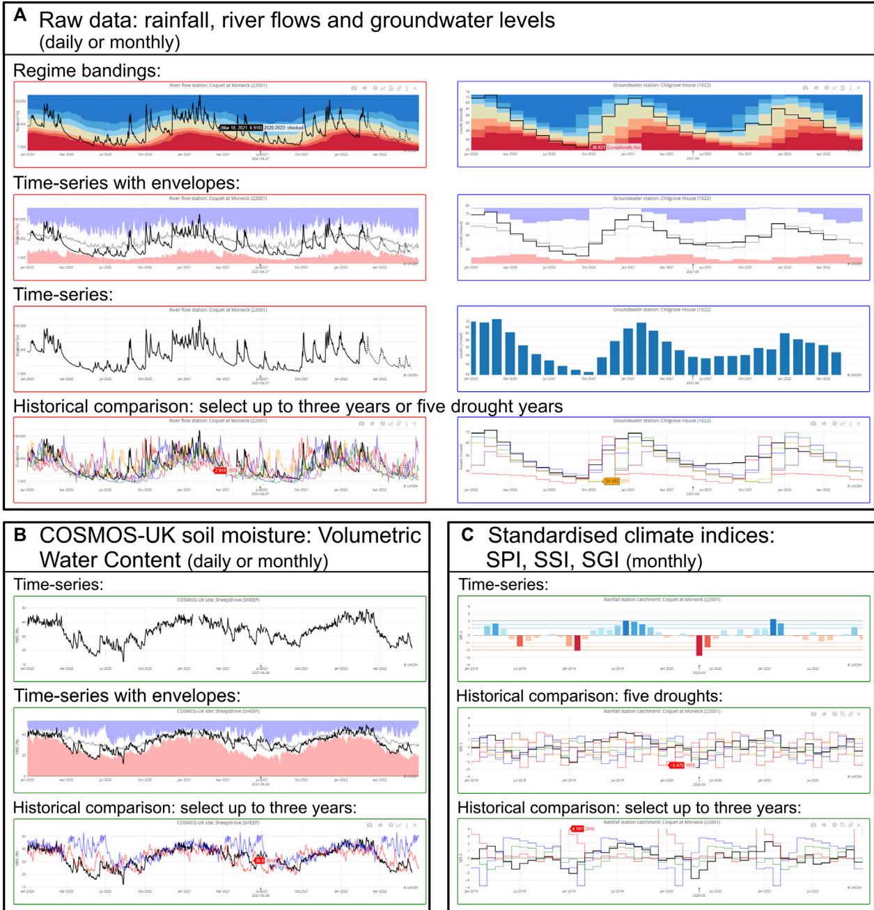
FIGURE 4 | Examples of plot types in the UK Water Resources Portal showing (A) daily river flow data for the River Coquet at Morwick and monthly groundwater levels at Chilgrove House, (B) soil moisture data for the COSMOS-UK site at Sheepdrove, and (C) SPI-3 for the Coquet catchment.
