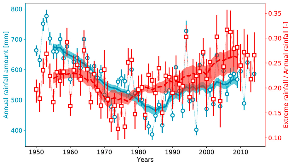
Fig. 2. Mean annual rainfall (left axis) and extreme rainfall (defined as daily rainfall that occurs on average two times a year) as a proportion of annual rainfall (right axis) over the Central Sahelian box [11–16°N, 2°W–5°E; see Fig. 1] during the 1950–2014 period (red symbols and corresponding 11-year moving mean shown with a red line; the cyan symbols and lines indicate the annual rainfall amounts). Data and method is from Panthou et al. (2014, 2018). (For interpretation of the references to colour in this figure legend, the reader is referred to the Web version of this article.)
