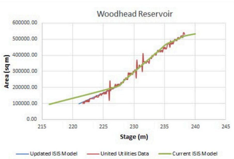
Figure A4.3.2 Comparison between current (green) and updated (blue) stage-area curves for FM (ISIS) models and United Utilities data (red) for Woodhead Reservoir. (Source: CH2M (2016))
