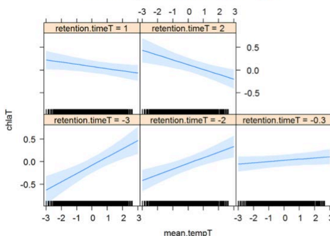
mean.temp*retention.timeT effect plot
