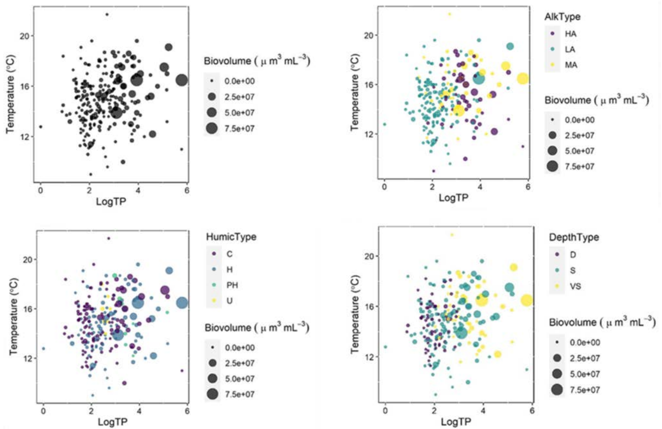
Figure A4.3 Relationship between cyanobacterial biovolume, log e total phosphorus (LogTP) concentrations and water temperature in all Scottish lochs with sufficient data (top left) and in lochs with different typologies. Alkalinity type [AlkType) – top right; Humic type – bottom left; Depth type – bottom right). Abbreviations are: HA = High Alkalinity; LA = Low Alkalinity; MA = Medium Alkalinity; C = clear; H = Humic; PH = Polyhumic; Humic; U = Unknown; D = Deep; S = Shallow; VS = Very Shallow. © UKCEH. Contains SEPA data © Scottish Environment Protection Agency and database right 2021. All rights reserved.
