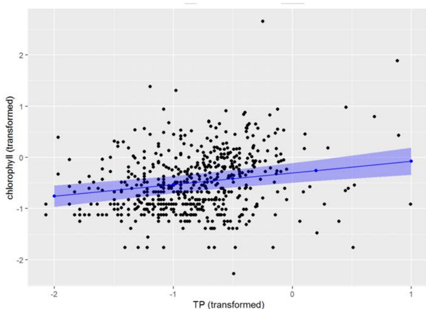
Figure A5.7. Relationship between Loge transformed TP and chlorophyll-a concentrations in deep lochs showing the modelled best fit. © UKCEH. Contains SEPA data © Scottish Environment Protection Agency and database right 2021. All rights reserved.
