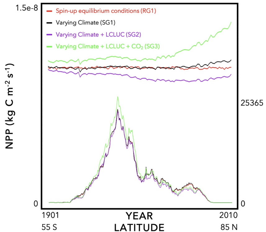
Figure 4. Inter-simulation visual diagnostics for M&T MIP Phase I experiments show how a single model changes output among different experiments. Here, we show output (e.g., Net Primary Productivity, NPP, for HyLand) from four experiments: (1) spin-up equilibrium conditions (RG1); (2) varying climate (SG1); (3) varying climate and land use/land cover change (LCLUC) (SG2); and (4) varying climate, LCLUC, and CO 2 (SG3). The top set of lines (primary y-axis) is the annual average from 1901 to 2010. The bottom set of lines (secondary y-axis) is the latitudinal/zonal sum from 55°S to 85°N.
