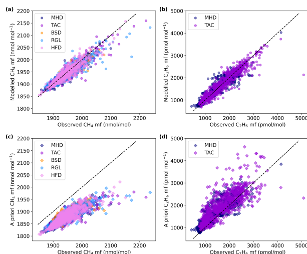
Figure F1. Scatter plot comparing mole fraction observations of methane (left, a, c ) and ethane (right, b, d ) as used in this study (2015–2019) to posterior mean modelled estimates of these values, made using the joint methane–ethane inversion ( a, b ). Comparison with a priori estimates of mole fraction concentrations made by combining the a priori flux maps with the transport model are also given ( c, d ) to show how the joint model improves the fit to observations. Points are colour-coded by site, with the locations of these sites given in Fig. A1.
