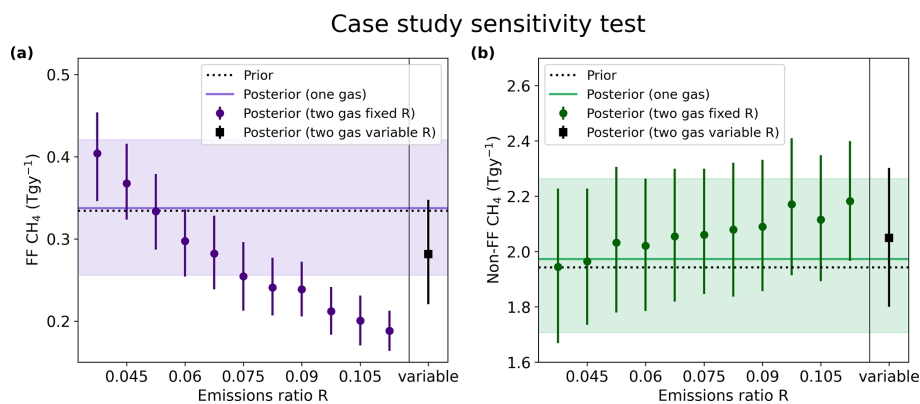
Figure 6. Posterior UK methane fluxes for May 2015, expressed as means and 95 % uncertainty intervals. Methane-only model (solid line and shading) and joint methane–ethane model (dots and error bars) with either a fixed emission ratio or a variable emission ratio (rightmost value in both a and b ). FF fluxes on the left in purple ( a ) and non-FF fluxes on the right in green ( b ). The a priori mean fluxes are given as dashed grey lines.
