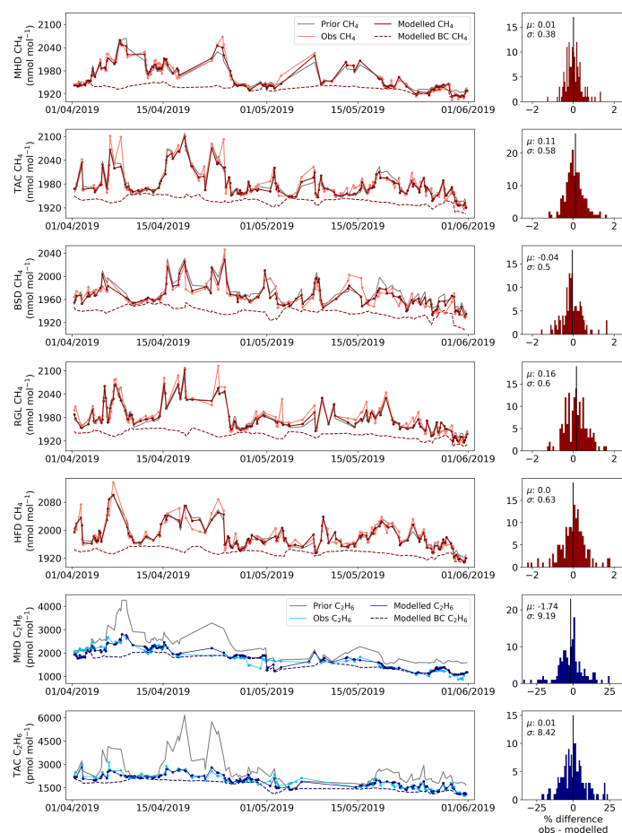
Figure 3. Left: observations and modelled observations (dots and solid lines) of methane (red) and ethane (blue) from the UK DECC network for April–May 2019. Modelled boundary condition (baseline) emissions are also given (dashed line) along with the a priori modelled concentrations (grey). Note the different scales for each site and for each gas. Right: histograms showing the percentage differences between observed and modelled mole fractions are provided for each gas and site.
