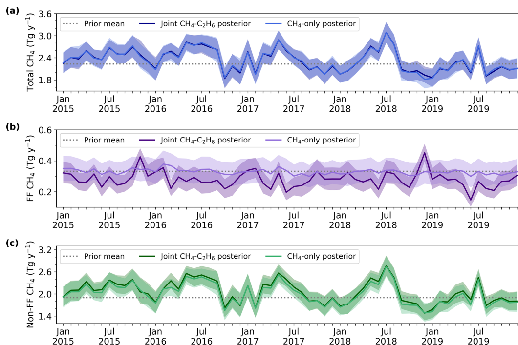
Figure 2. Posterior monthly UK methane emissions in teragrams per year ( \text{Tg yr}^{-1} ). Total (a, blue), FF (b, purple) and non-FF (c, green), expressed as posterior means and 95 % uncertainty intervals of these PDFs. Methane-only model output (lighter shade line and shading) and joint methane–ethane model output (darker shade line and shading) both shown for comparison. A priori mean fluxes from the UKGHG model are given as a grey dashed line.
