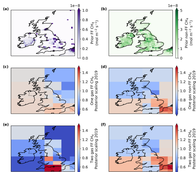
Figure 4. A priori emissions and 2019 annual mean posterior emission scaling factors for UK FF (left, a , c , e ) and non-FF (right, b , d , f ) methane fluxes. A priori fluxes from the UKGHG model, as described in the text, are given at the resolution of the transport model ( a , b ). Posterior mean flux scaling factors from the methane-only ( c , d ) and joint ethane–methane ( e , f ) inverse models are given at the coarser resolution of the transport model. Red and blue indicate a scaling up or down, respectively, of the a priori estimate.
