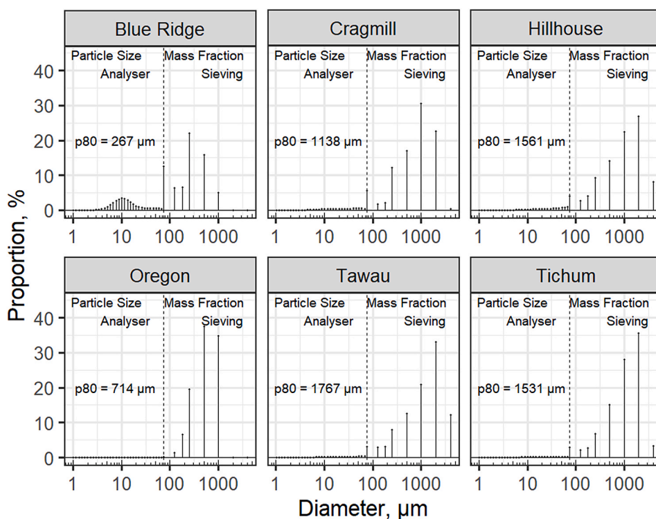
Fig. 3. Basalt particle size distributions, as determined with a particle analyser ( <75 \mu\text{m} ) ( n \geq 5 samples per basalt) and from mass fraction sieving ( >75 \mu\text{m} ) ( n = 4 samples per basalt). Analysis from the particle size analyser provides the proportion of total concentration of particles, while mass fraction sieving provides the proportion of the total weight. The cumulative density functions for each basalt, from which the p80 was determined, are given in the Supplementary Information (Fig. S3).
