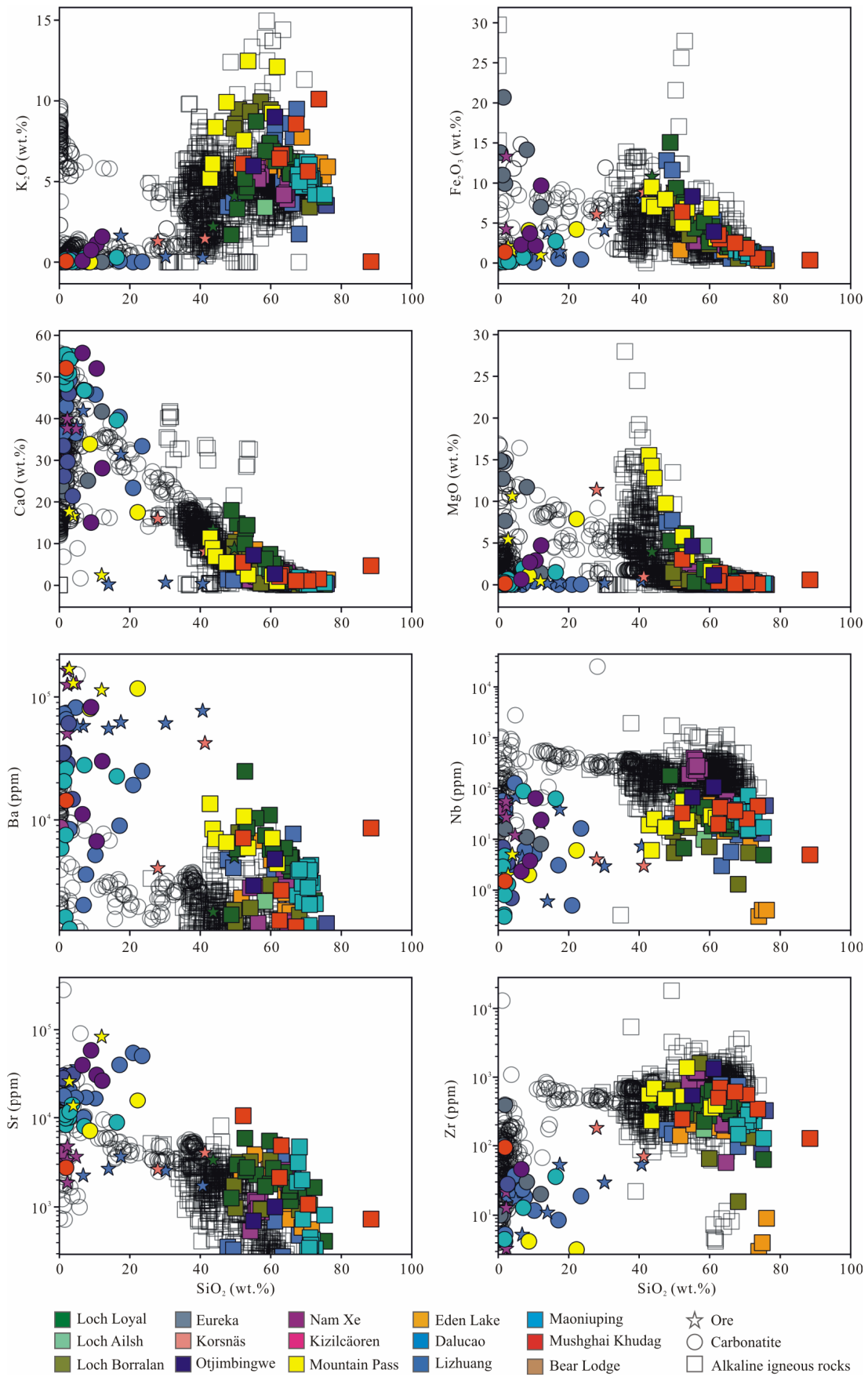
Figure 7. Plots of selected major oxides and trace elements against SiO 2 for alkaline-carbonatite complexes described in the text. Previously unpublished data for Kizilcäoren, Eureka and Loch Borralan from Table 1: all other post-collisional data (filled, coloured symbols) from published references cited in the text and shown in Table S1. Comparative data for the East African Rift (open symbols) downloaded from GEOROC.
