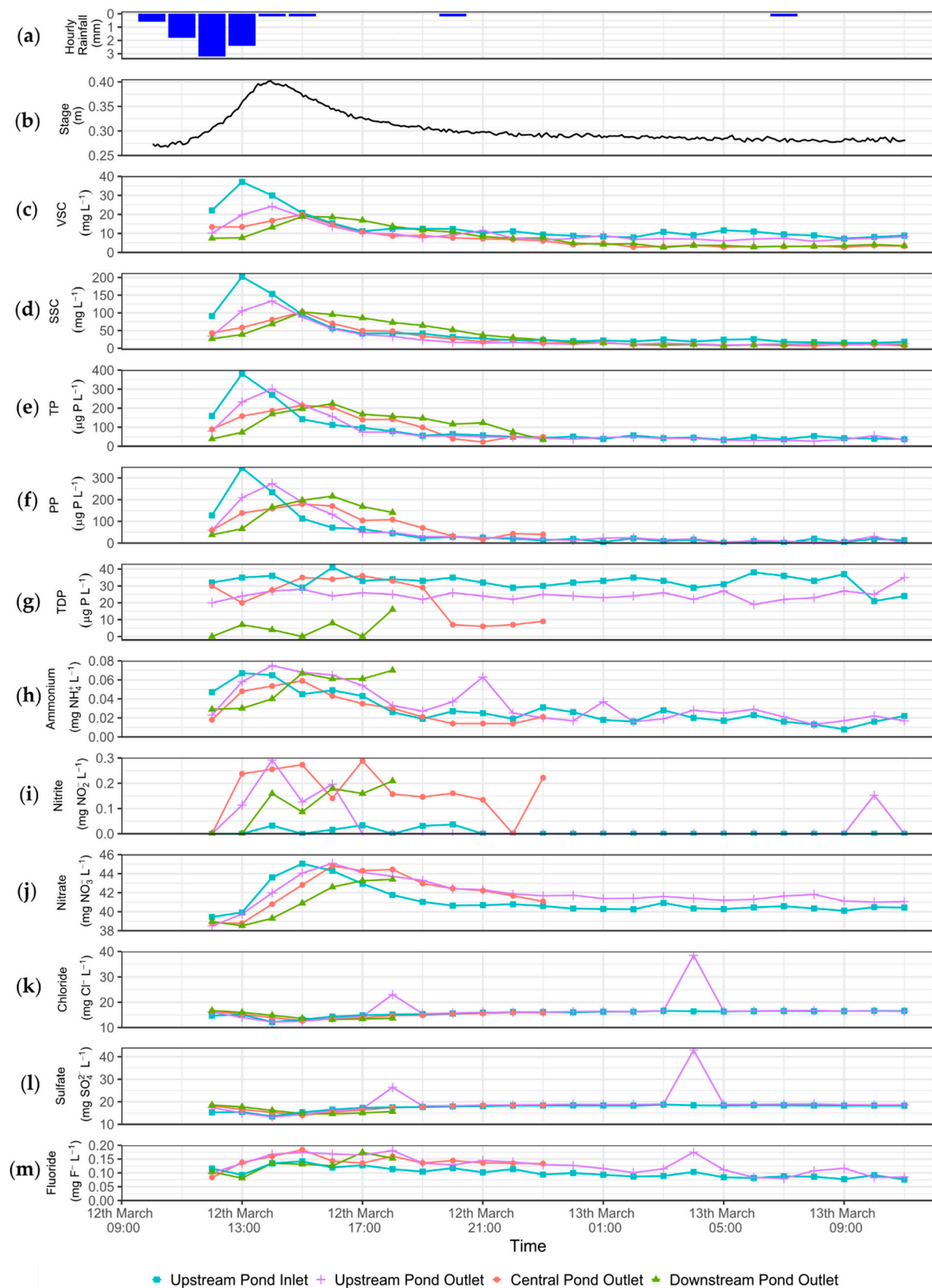
Figure 4. Timeseries during a storm event on 12/13 March 2019 showing: (a) hourly rainfall (mm); (b) stage (m) in the Central Pond; and concentrations of water quality determinands: (c) VSC and (d) SSC ( \text{mg L}^{-1} ); (e) TP, (f) PP, and (g) TDP ( \mu\text{g P L}^{-1} ); (h) ammonium ( \text{mg NH}_4^+ \text{L}^{-1} ); (i) Nitrite ( \text{mg NO}_2^- \text{L}^{-1} ); (j) Nitrate ( \text{mg NO}_3^- \text{L}^{-1} ); (k) chloride ( \text{mg Cl}^- \text{L}^{-1} ); (l) Sulfate ( \text{mg SO}_4^{2-} \text{L}^{-1} ) and (m) Fluoride ( \text{mg F}^- \text{L}^{-1} ) at each pond inlet/outlet sampling site.
