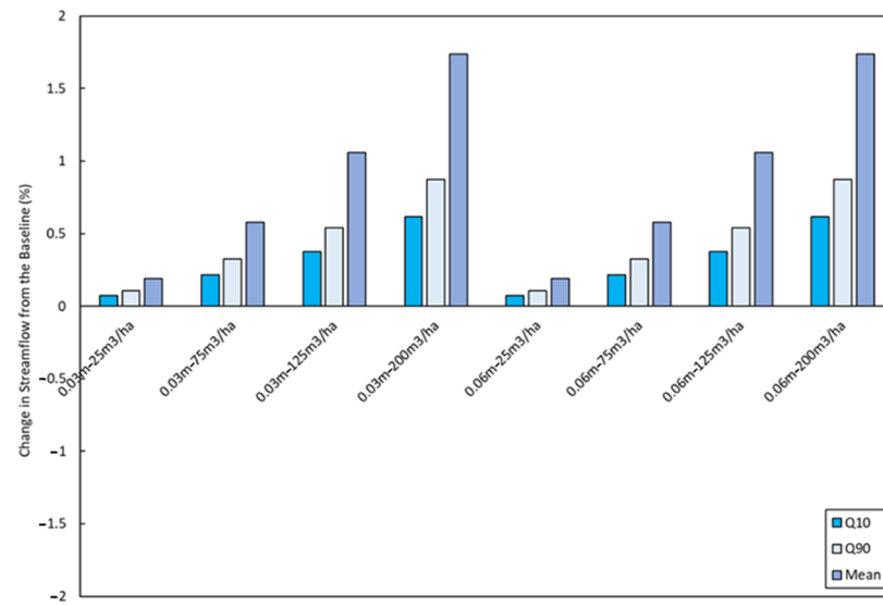
Figure A3. The change in the Q 10 , Q 90 and mean simulated streamflow from the baseline with the inclusion of farm bunds of various density and dimensions (Table A1).
