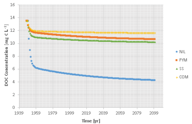
Figure 3. Estimated DOC concentration time trends in ZOFE topsoil (20 cm) for the treatments NIL, FYM, SS and COM.
