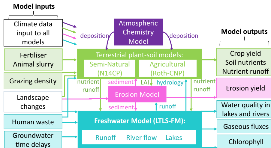
Fig. 1. Schematic of the full LTLS-IM, with arrows indicating where output from one model or dataset is input to another. Freshwater model (LTLS-FM) components are shown in blue. (For interpretation of the references to colour in this figure legend, the reader is referred to the web version of this article.)
