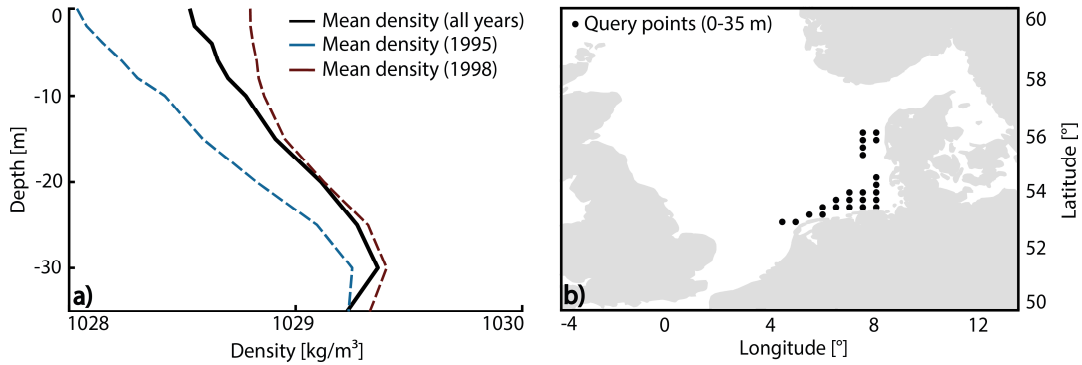
Figure 9: (a) Vertical profiles of potential density as averaged over all query points in (b) at depths from 0 to 35 m for the years 1958 to 2013 (black), the year 1995 (blue) and the years 1998 (red). The two selected years feature the greatest deviation from the mean density profile.
