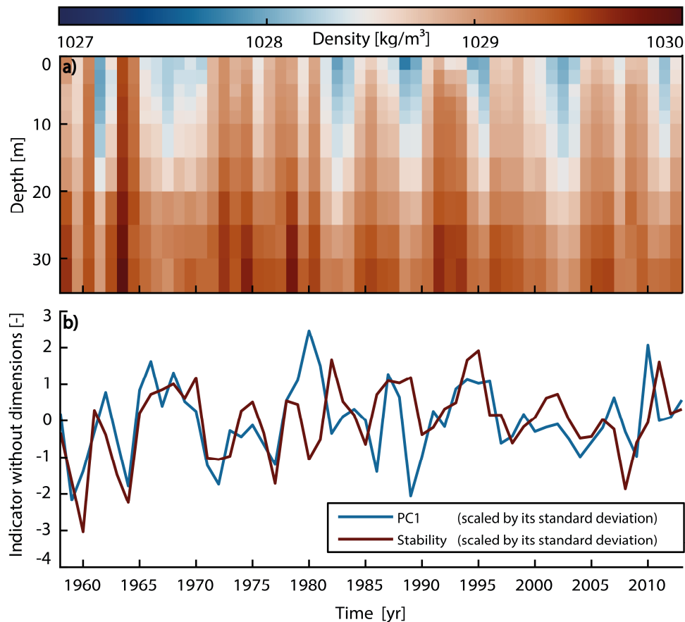
Figure 10: (a) Spatially averaged density profiles (0–35 m) from the query area in Figure 9-b spanning the period 1958 to 2013. (b) Comparison between PC1 changes and the stability index (see main text), where both time series were scaled by their standard deviation and adjusted for long-term trends.
