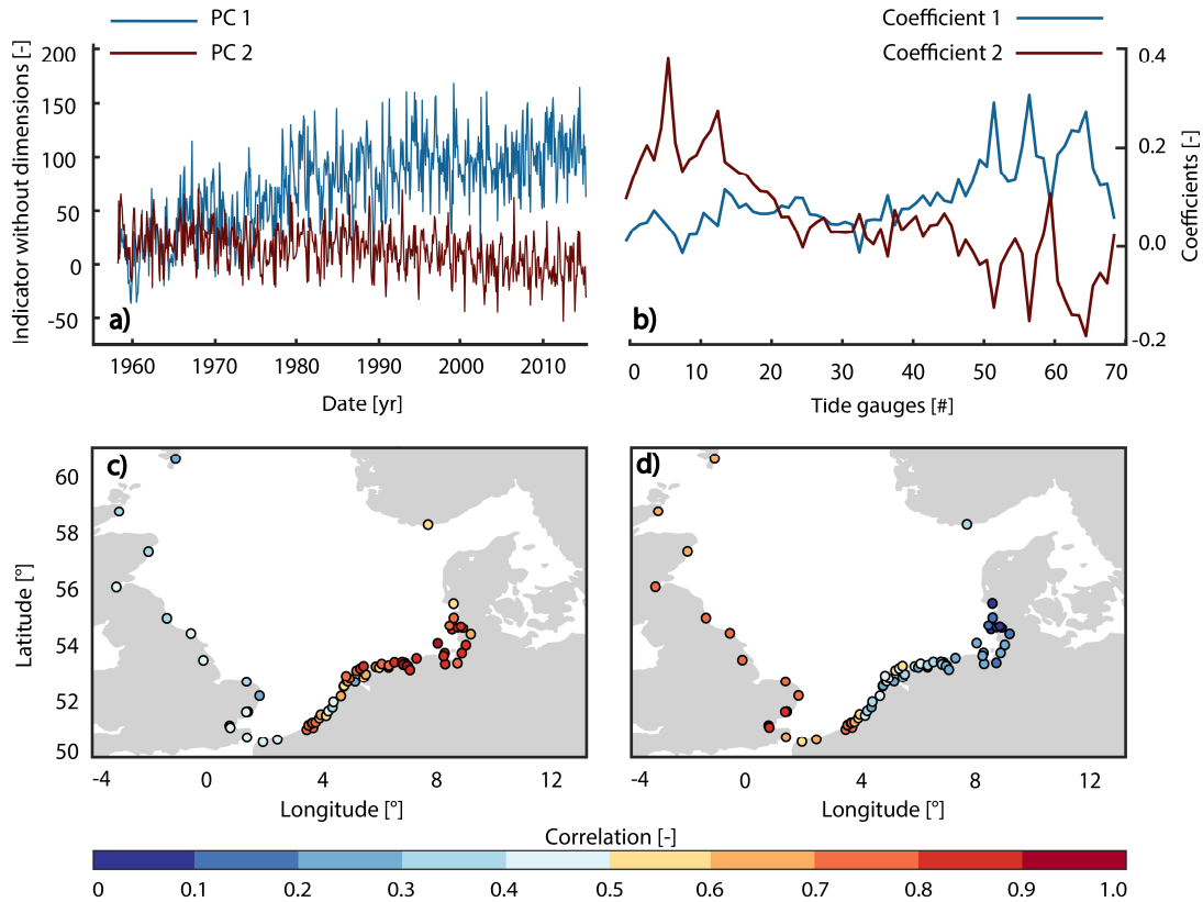
Figure 6: Results of the PCA. (a) Shown are time series of PC1, and PC2 and (b) their corresponding spatial patterns. Panels (c) and (d) map the correlations between observations and PC1 (c) and PC2 (d) for each site.
