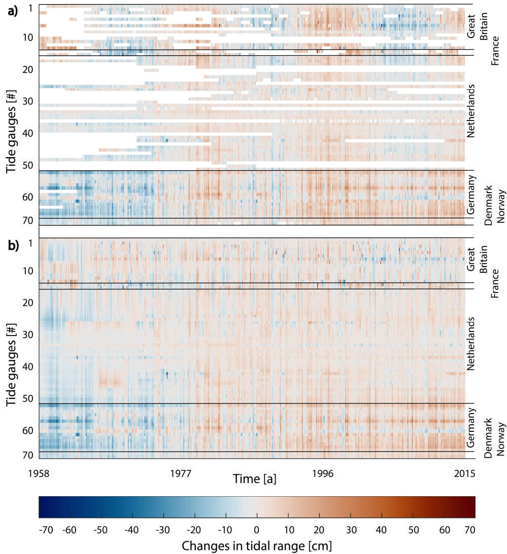
Figure 3: Changes in tidal range before (a) and after (b) applying ordinary kriging and removing the nodal cycle.
