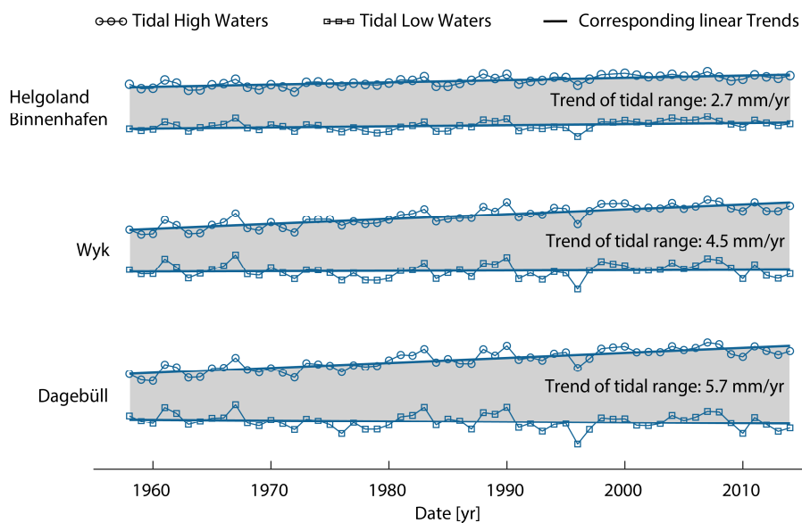
Figure 1: Time series of mean annual high and low tidal water levels for three exemplarily selected stations in the German Bight. For illustration purposes all records are shown with different artificial vertical offsets. The increase in the tidal range is illustrated for the three sites as grey shaded areas between high and low water level time series.
