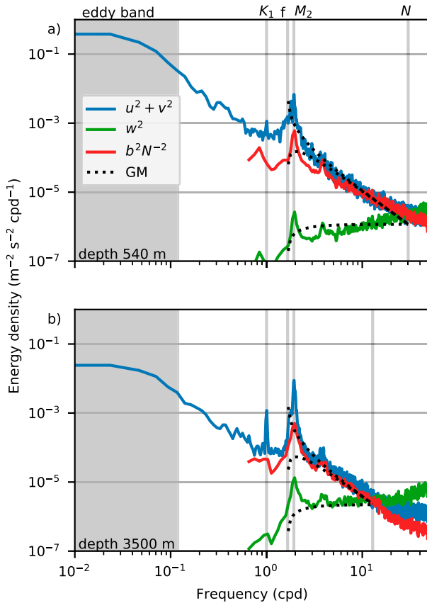
FIG. 4. Spectra from C mooring at depths of (a) 540 and (b) 3500 m of horizontal kinetic energy ( u^2 + v^2 ), potential energy ( b^2 N^{-2} ), and vertical kinetic energy ( w^2 ). Garrett–Munk spectra are added as dashed lines, using the formulation described by Cairns and Williams (1976). Solid vertical lines indicate the K_1 and M_2 tidal constituents, the Coriolis frequency f , and the buoyancy frequency N . The shaded region on the left denotes the eddy portion of the spectrum, which corresponds to periods longer than about 5 days, set by the averaging period used in the analysis.
