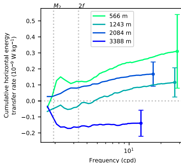
FIG. 6. Cumulative sums of the horizontal energy transfer rate in frequency for each depth level. The error bars denote the 95% confidence interval on the final point.
