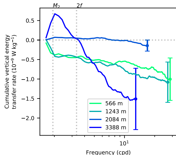
FIG. 9. Cumulative sums of the vertical energy transfer rate in frequency for each depth level. The error bars denote the 95% confidence interval on the final point.
