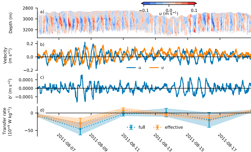
FIG. 10. Time series of (a) high-pass zonal velocity from the downward-looking long-ranger ADCP, (b) zonal and meridional velocity from the deepest current meter, (c) buoyancy, and (d) the full and effective vertical energy transfer rates.
