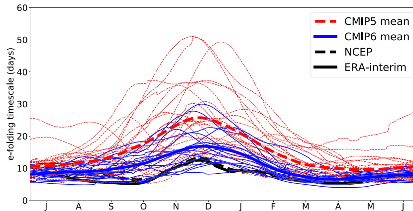
Figure 5. SAM_{EOF} decorrelation timescale as a function of season. CMIP5 models are shown in thin red dashed lines and CMIP6 models in solid blue lines. The multi-model means are thicker red dashed and solid blue lines for CMIP5 and CMIP6, respectively, while ERA-Interim (solid black) and NCEP reanalysis (dashed black) values are also shown for comparison.
