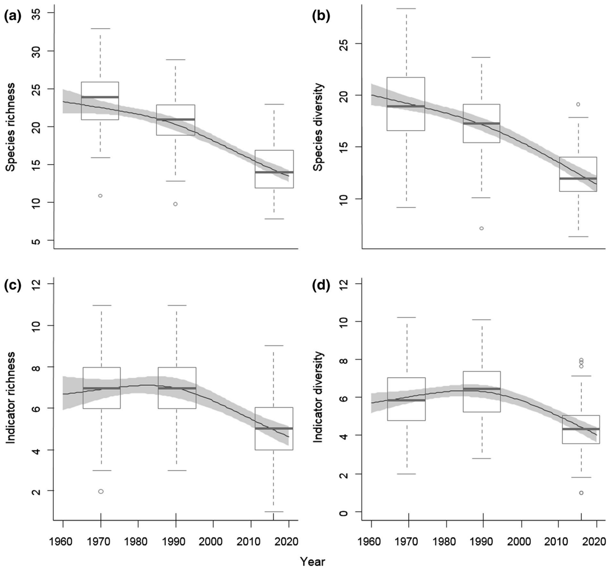
Fig. 2 Boxplots of a species richness, b species diversity, c indicator richness and d indicator diversity, for 115 quadrats (20 cm × 20 cm) in 1970, 1990 and 2016 at Parsonage Down.
