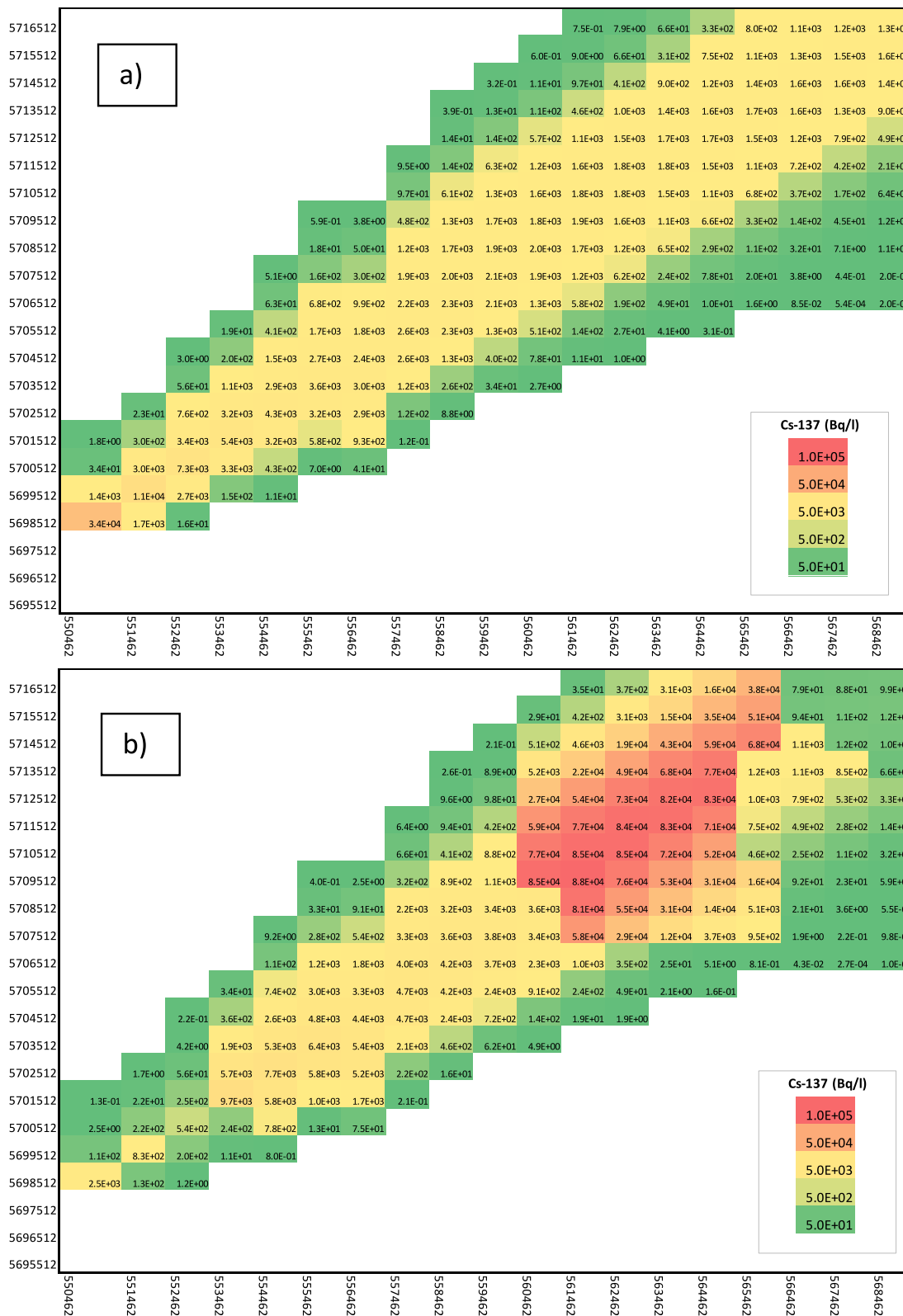
Fig. 5. Predictions of 137 Cs activity concentrations in milk (Bq l -1 ) at 5 years for (a) FDMT and (b) process based (“Absalom”) using the soil categorisations as described earlier (Fig. 2). Each cell covers an area of 1 km 2 . Values in the legend key represent maxima for each colour band.
