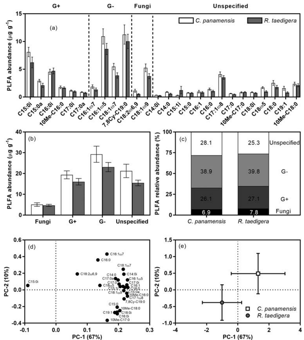
Fig. 2 (a) PLFA biomarker abundance for C. panamensis and R. taedigera . (b) Net abundance of fungal, Gram positive (G+), Gram negative (G-) and unspecified PLFA biomarkers. (c) Relative abundance of fungal, Gram positive, Gram negative and unspecified PLFA biomarkers. (d) PCA loadings for PLFA biomarkers. (e) PCA scores for PLFA biomarkers. Means \pm one SE ( n = 5 )
