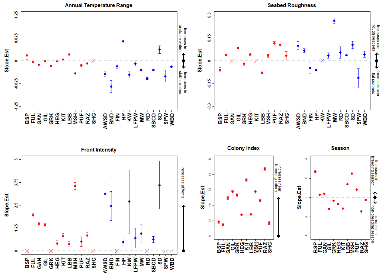
Figure 2: Summary of linear relationships between species and environmental variables in the North-East Atlantic, as quantified using a binomial (annual temperature range, colony index, season) or Poisson (seabed roughness, front intensity) GEE-GLM. Points indicate slope estimates, whereas lines indicate standard errors around this estimate. The dashed line indicates a slope estimate of 0. Crosses indicate when a relationship was not identified. Information on environmental variables is in Table 4. Cetaceans are shown in blue, and seabirds are shown in red. Species codes are described in Table 1.
