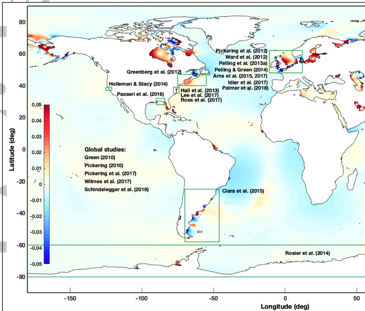
Figure 8: Approximate location of the studies that have modelled future changes in tides, overlaid on a map of changes in mean high water in m yr -1 from Pickering et al. (2017).
