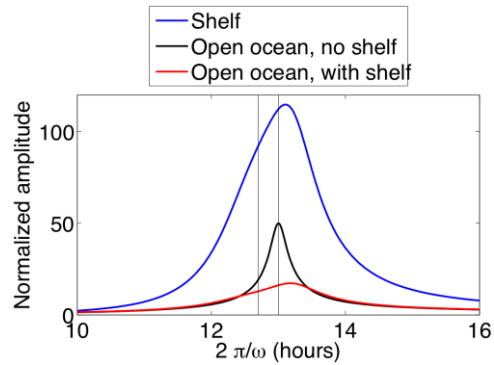
M_2 amplitudes in blocked and unblocked Hudson Strait experiments
