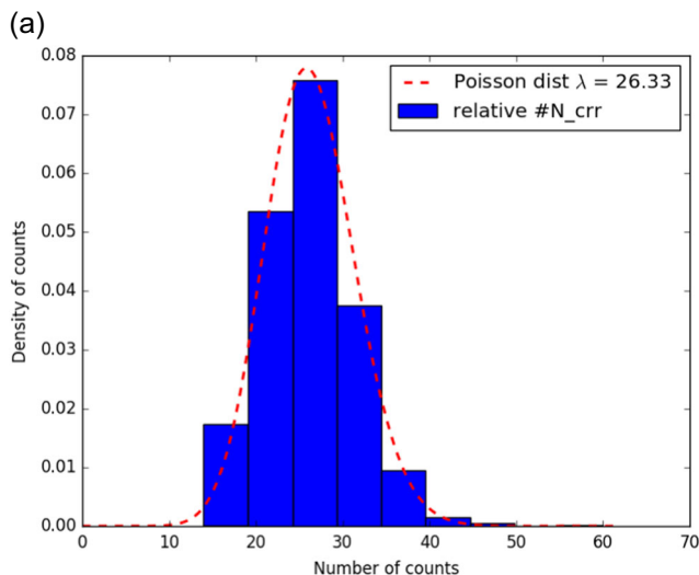
FIGURE 1 An example measurement from the cosmic-ray sensor (a) distribution of fast neutron counts, (b) evolution of the count rate and measurement uncertainty over time, black dots denote 1 out of 20 sensor readings for illustrative purposes [Color figure can be viewed at wileyonlinelibrary.com]
