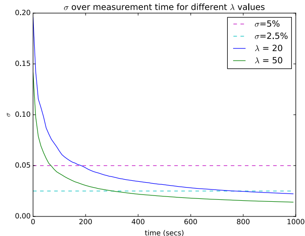
FIGURE 2 Measurement uncertainty \sigma over time for different \lambda values and sample thresholds for the adaptive measurement interval regime [Color figure can be viewed at wileyonlinelibrary.com]
