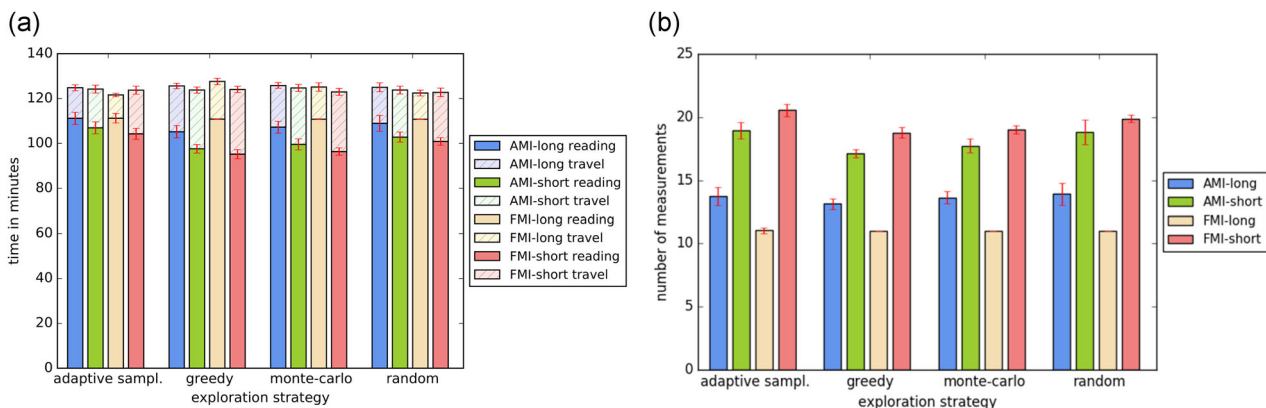
FIGURE 6 High-gradient synthetic scenario. Comparison of different sampling regimes and exploration strategies: (a) Measurement and travel times, (b) Number of samples taken. Average results over 30 runs with, error bars representing standard deviation for each case [Color figure can be viewed at wileyonlinelibrary.com]
