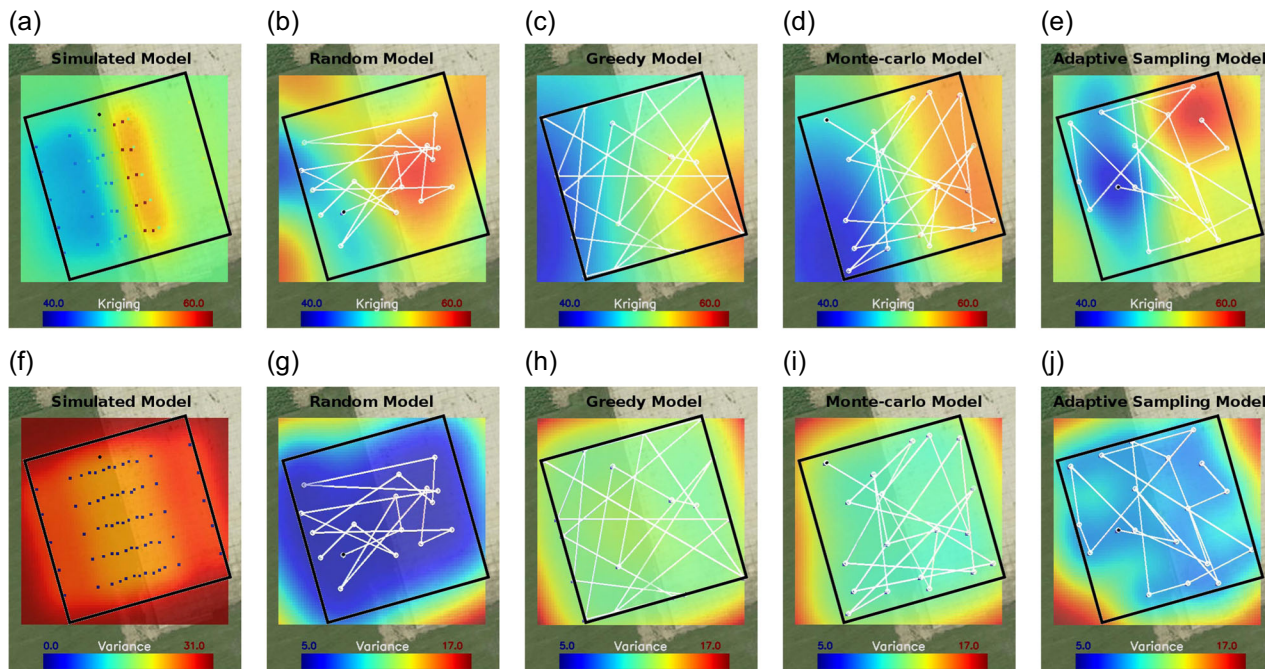
FIGURE 13 Simulated model: exploration outputs and robot trajectories. The kriging output (top row) and variance (bottom row) for the (a,f) full model, (b,g) Random, (c,h) Greedy, (d,i) Monte Carlo, and (e,j) Adaptive sampling strategies [Color figure can be viewed at wileyonlinelibrary.com]
