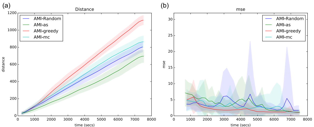
FIGURE 12 Simulated scenario. Performance for different strategies using adaptive measurement intervals in terms of (a) distance and (b) mean square error. Shaded areas represent standard deviation over 30 runs [Color figure can be viewed at wileyonlinelibrary.com]
