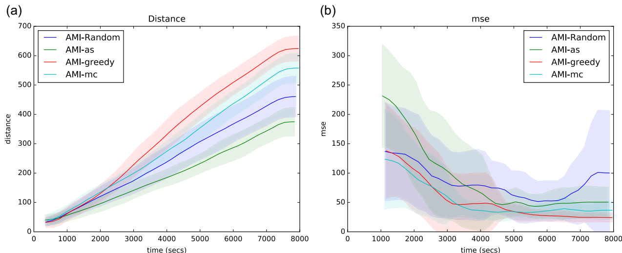
FIGURE 10 High-gradient synthetic scenario. Performance for different strategies using adaptive measurement intervals in terms of (a) distance, and (b) mean square error. Average results over 30 runs, shaded areas represent standard deviation for each case [Color figure can be viewed at wileyonlinelibrary.com ]
