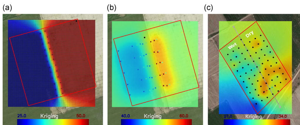
FIGURE 5 The high-gradient synthetic model generated from the airfield (a), the simulated model (b), and the validation model generated from the wheat stubble field (c) [Color figure can be viewed at wileyonlinelibrary.com ]
