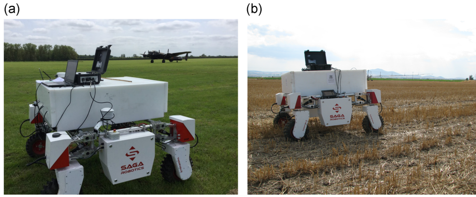
FIGURE 3 The Thorvald robot equipped with a cosmic-ray sensor during data collection at an airfield at the Lincolnshire Aviation Heritage Center in East Kirkby, UK (left); a wheat stubble field near Volos, Greece (right) [Color figure can be viewed at wileyonlinelibrary.com ]
