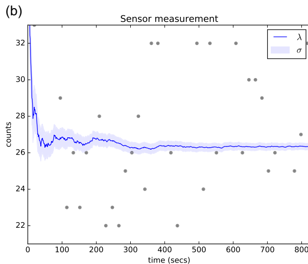
FIGURE 1 An example measurement from the cosmic-ray sensor (a) distribution of fast neutron counts, (b) evolution of the count rate and measurement uncertainty over time, black dots denote 1 out of 20 sensor readings for illustrative purposes [Color figure can be viewed at wileyonlinelibrary.com]
