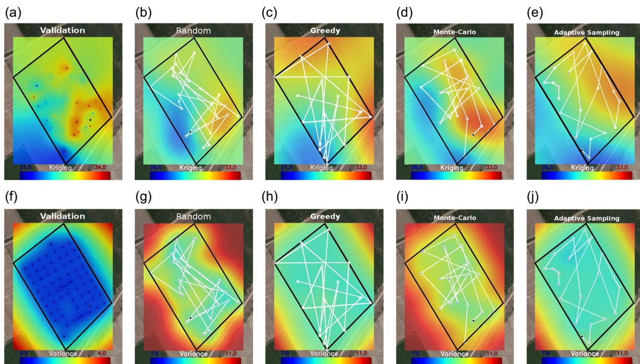
FIGURE 14 Validation model. Exploration outputs and robot trajectories. The kriging output (top row) and variance (bottom row) for the (a, f) full model, (b,g) Random, (c,h) Greedy, (d,i) Monte Carlo, and (e,j) Adaptive sampling strategies [Color figure can be viewed at wileyonlinelibrary.com]
