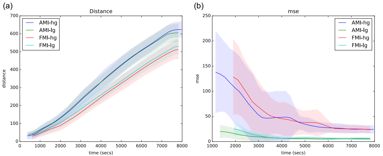
FIGURE 8 Comparison of performance of long fixed measurement interval and adaptive measurement interval in synthetic scenarios low-gradient synthetic and high-gradient synthetic in terms of (a) distance, and (b) mean square error. Average results over 30 runs, shaded areas represent standard deviation for each case [Color figure can be viewed at wileyonlinelibrary.com ]
